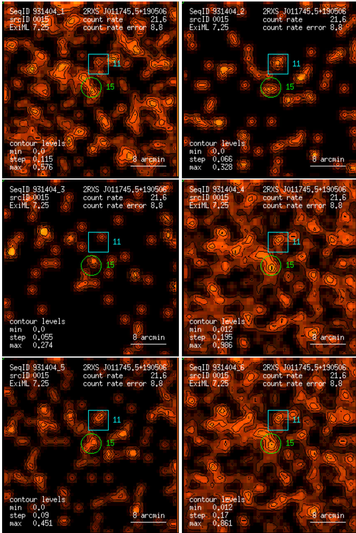
Figure 15: RASS 931404: detection 0015: band rate images, Gaussian filter: (1) PSPC channels 11 – 41, (2) 52 – 90, (3) 91 – 201, (4) 11 – 235, (5) 52 – 201, (6) 11 – 201. Broad band rates in counts/ks. Band rate contour levels in counts/ks/arcmin 2 .
