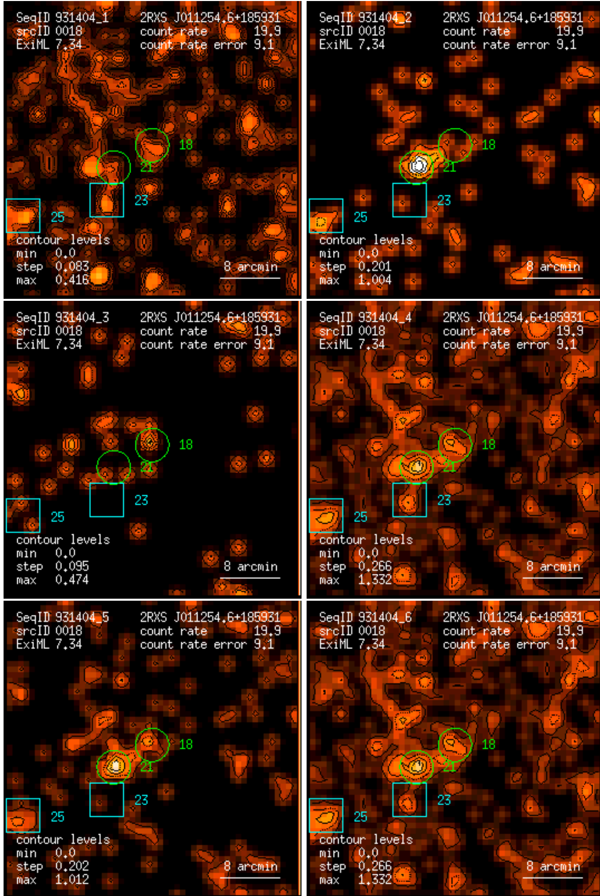
Figure 18: RASS 931404: detection 0018: band rate images, Gaussian filter: (1) PSPC channels 11 – 41, (2) 52 – 90, (3) 91 – 201, (4) 11 – 235, (5) 52 – 201, (6) 11 – 201. Broad band rates in counts/ks. Band rate contour levels in counts/ks/arcmin 2 .
