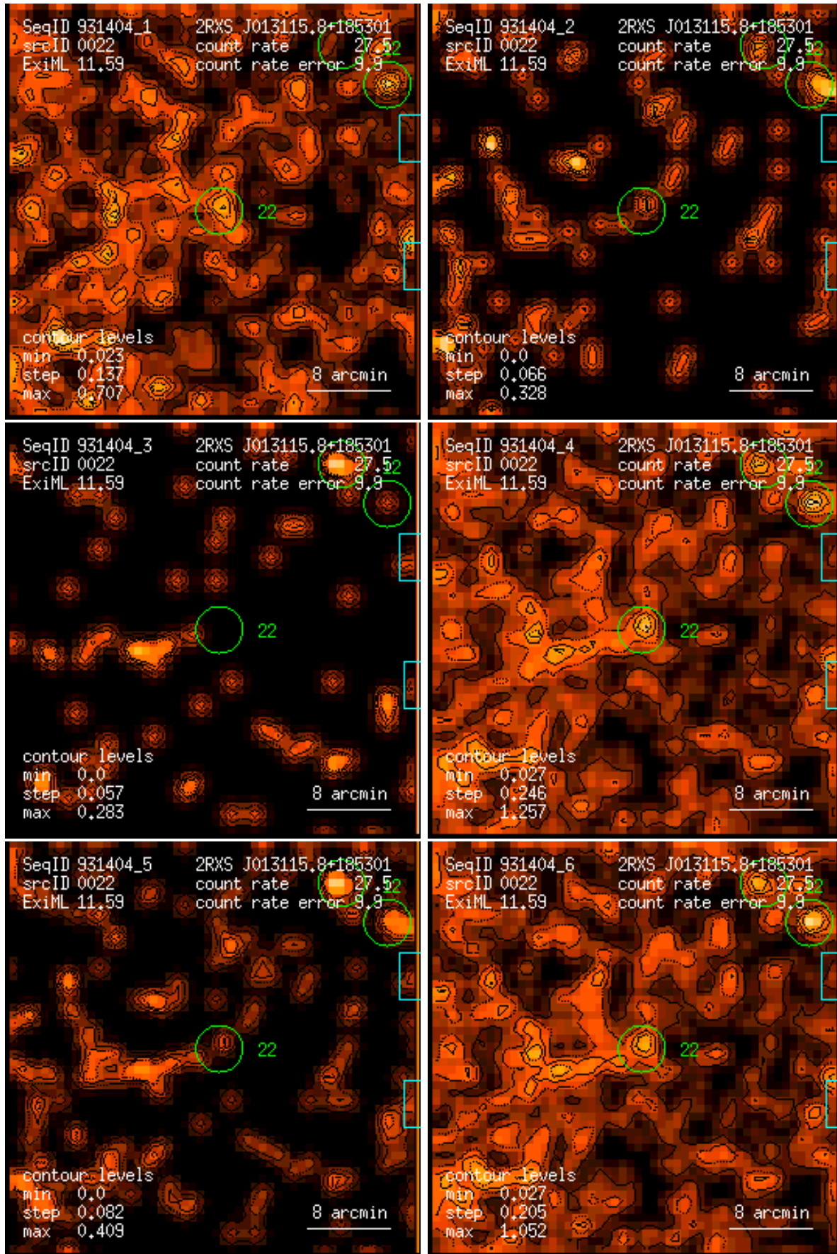
Figure 22: RASS 931404: detection 0022: band rate images, Gaussian filter: (1) PSPC channels 11 – 41, (2) 52 – 90, (3) 91 – 201, (4) 11 – 235, (5) 52 – 201, (6) 11 – 201. Broad band rates in counts/ks. Band rate contour levels in counts/ks/arcmin 2 .
