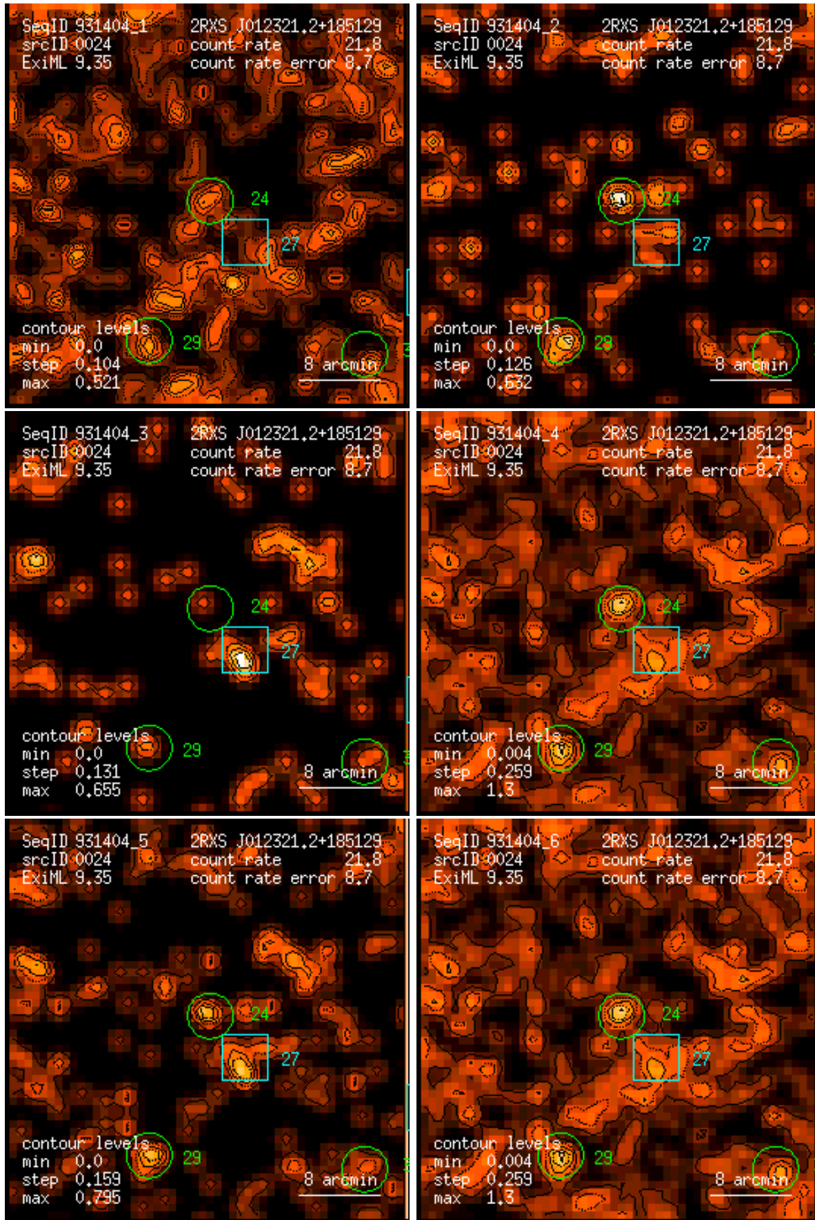
Figure 24: RASS 931404: detection 0024: band rate images, Gaussian filter: (1) PSPC channels 11 – 41, (2) 52 – 90, (3) 91 – 201, (4) 11 – 235, (5) 52 – 201, (6) 11 – 201. Broad band rates in counts/ks. Band rate contour levels in counts/ks/arcmin 2 .
