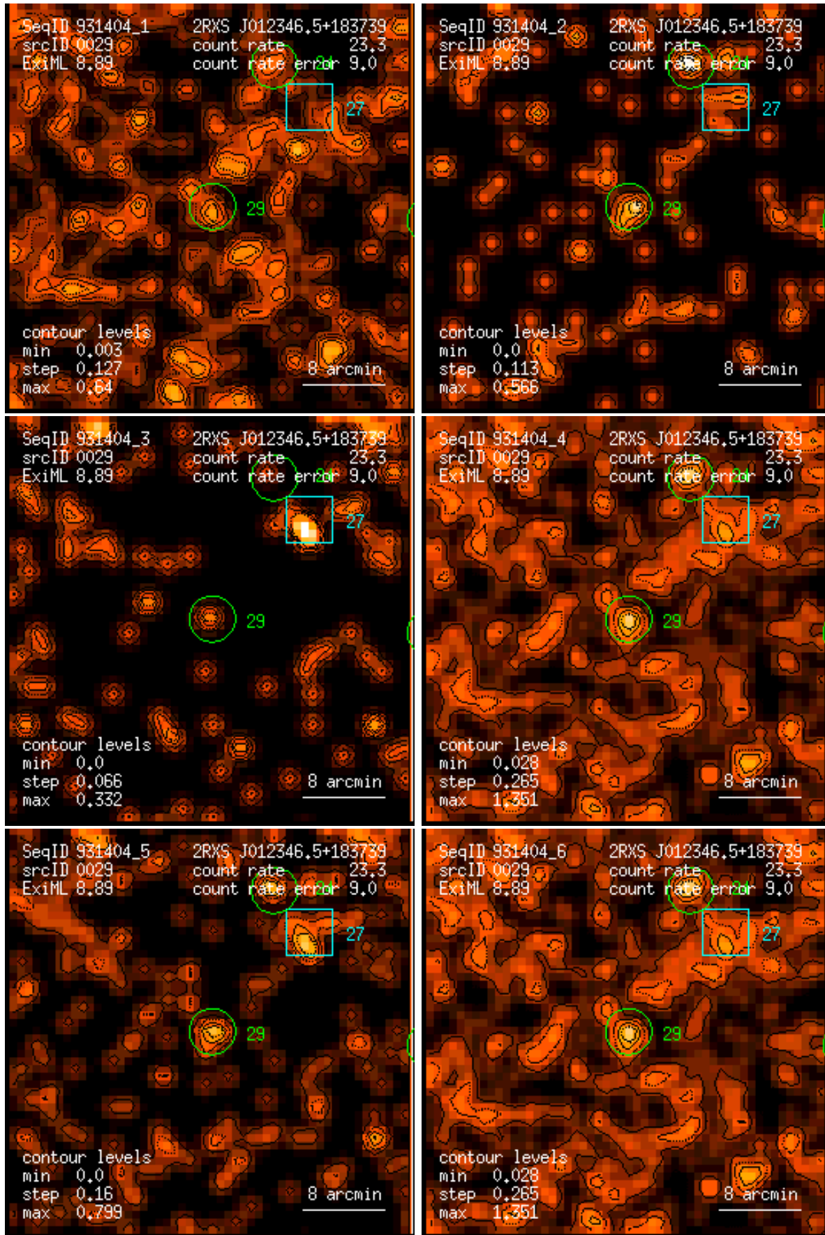
Figure 29: RASS 931404: detection 0029: band rate images, Gaussian filter: (1) PSPC channels 11 – 41, (2) 52 – 90, (3) 91 – 201, (4) 11 – 235, (5) 52 – 201, (6) 11 – 201. Broad band rates in counts/ks. Band rate contour levels in counts/ks/arcmin 2 .
