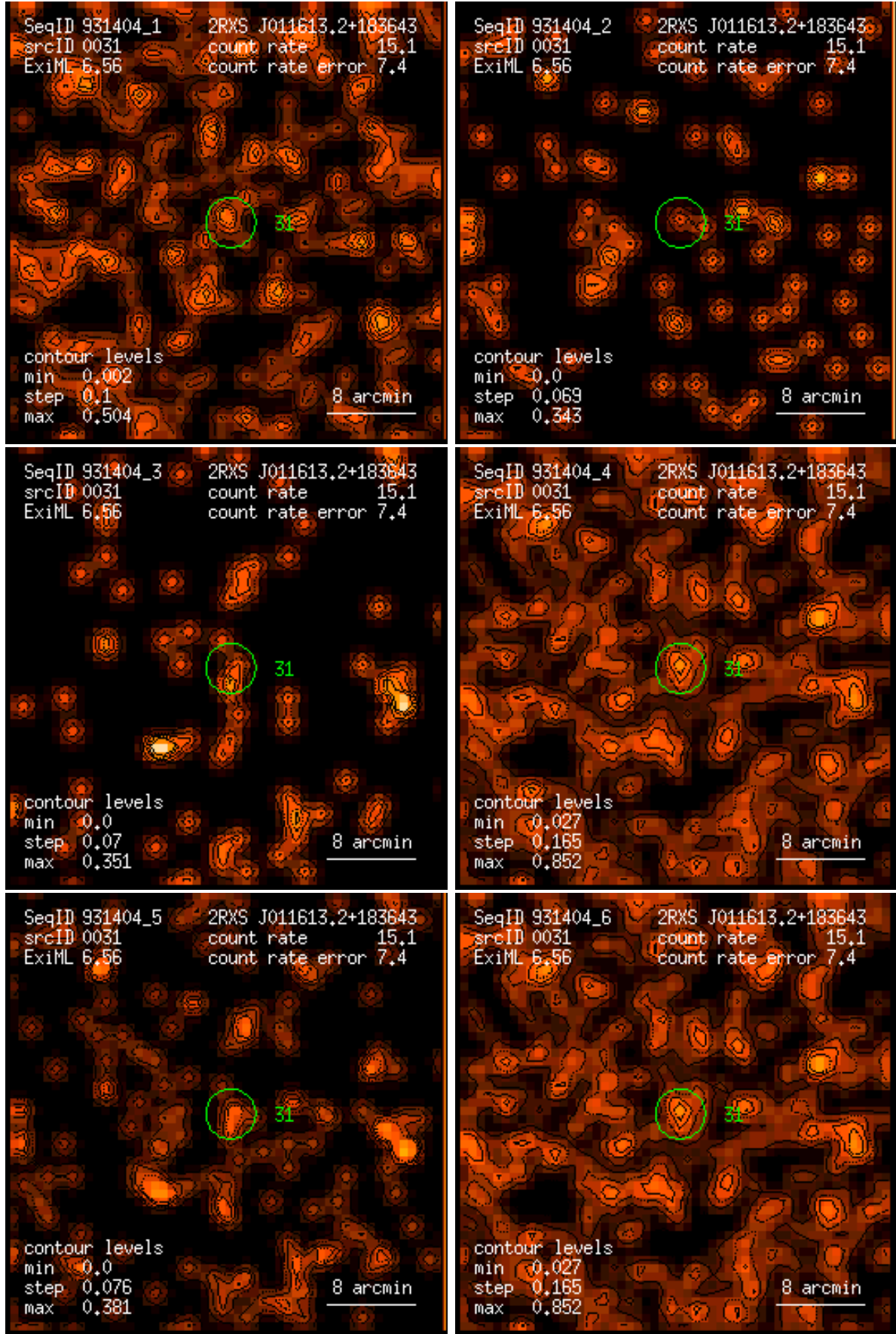
Figure 31: RASS 931404: detection 0031: band rate images, Gaussian filter: (1) PSPC channels 11 – 41, (2) 52 – 90, (3) 91 – 201, (4) 11 – 235, (5) 52 – 201, (6) 11 – 201. Broad band rates in counts/ks. Band rate contour levels in counts/ks/arcmin 2 .
