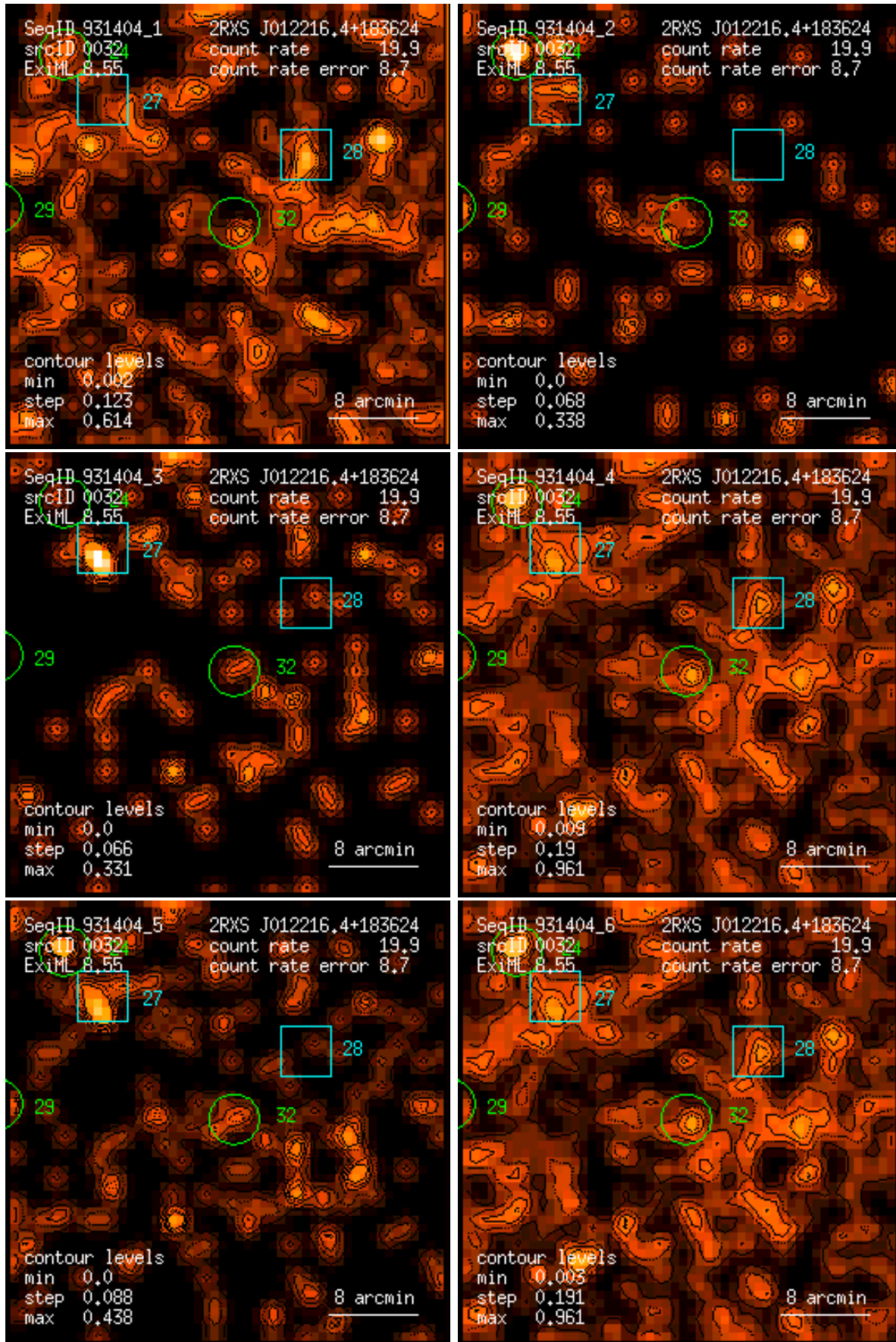
Figure 32: RASS 931404: detection 0032: band rate images, Gaussian filter: (1) PSPC channels 11 – 41, (2) 52 – 90, (3) 91 – 201, (4) 11 – 235, (5) 52 – 201, (6) 11 – 201. Broad band rates in counts/ks. Band rate contour levels in counts/ks/arcmin 2 .
