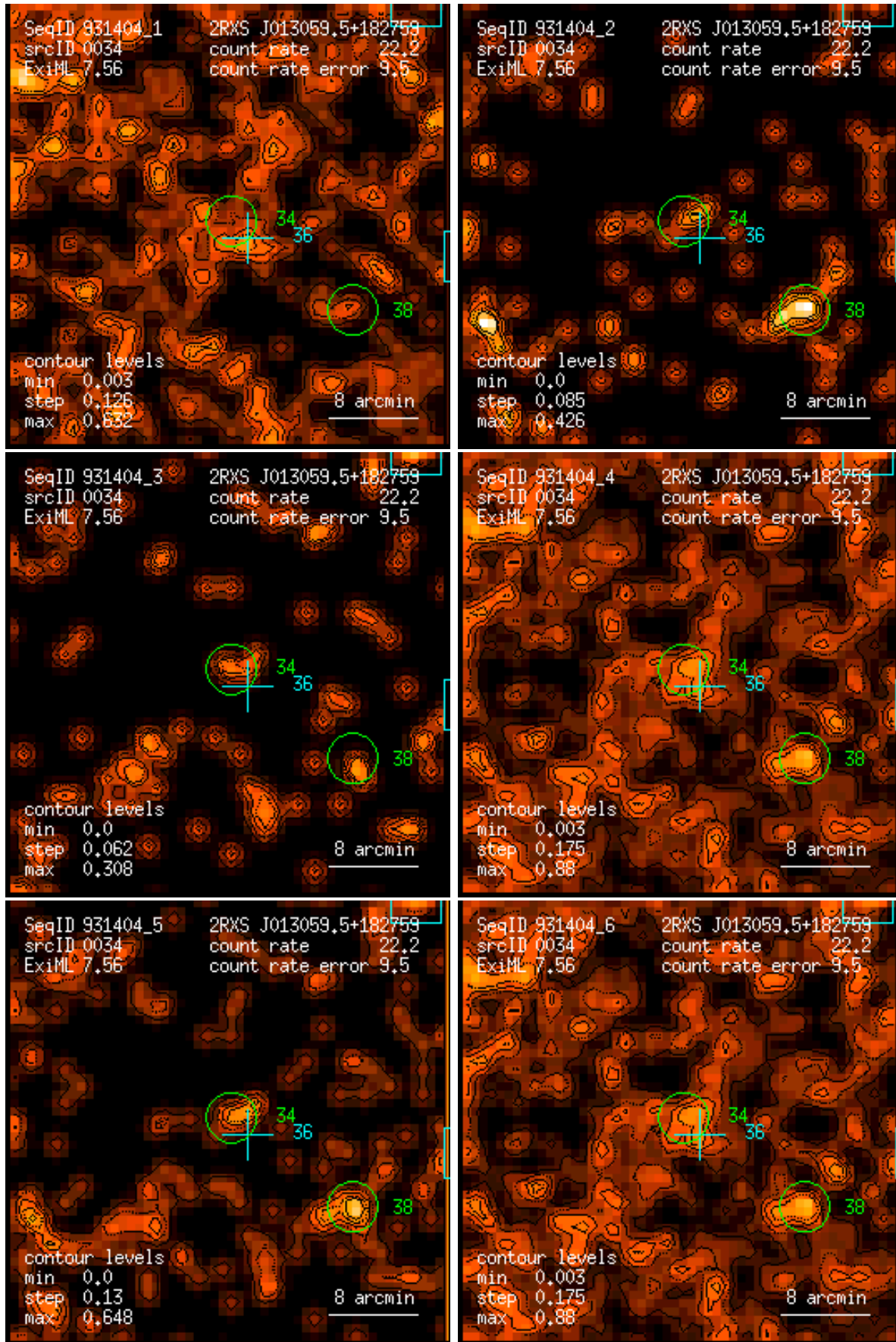
Figure 34: RASS 931404: detection 0034: band rate images, Gaussian filter: (1) PSPC channels 11 – 41, (2) 52 – 90, (3) 91 – 201, (4) 11 – 235, (5) 52 – 201, (6) 11 – 201. Broad band rates in counts/ks. Band rate contour levels in counts/ks/arcmin 2 .
