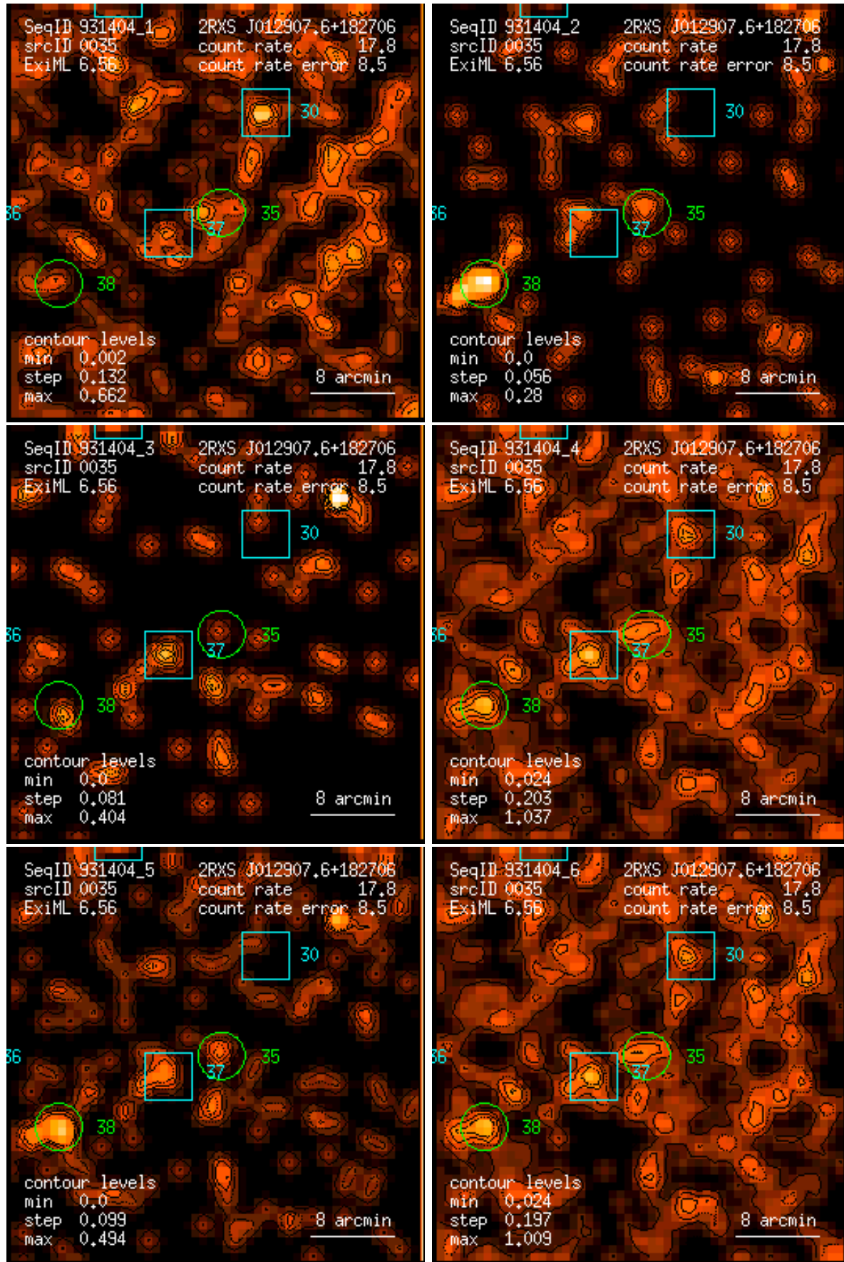
Figure 35: RASS 931404: detection 0035: band rate images, Gaussian filter: (1) PSPC channels 11 – 41, (2) 52 – 90, (3) 91 – 201, (4) 11 – 235, (5) 52 – 201, (6) 11 – 201. Broad band rates in counts/ks. Band rate contour levels in counts/ks/arcmin 2 .
