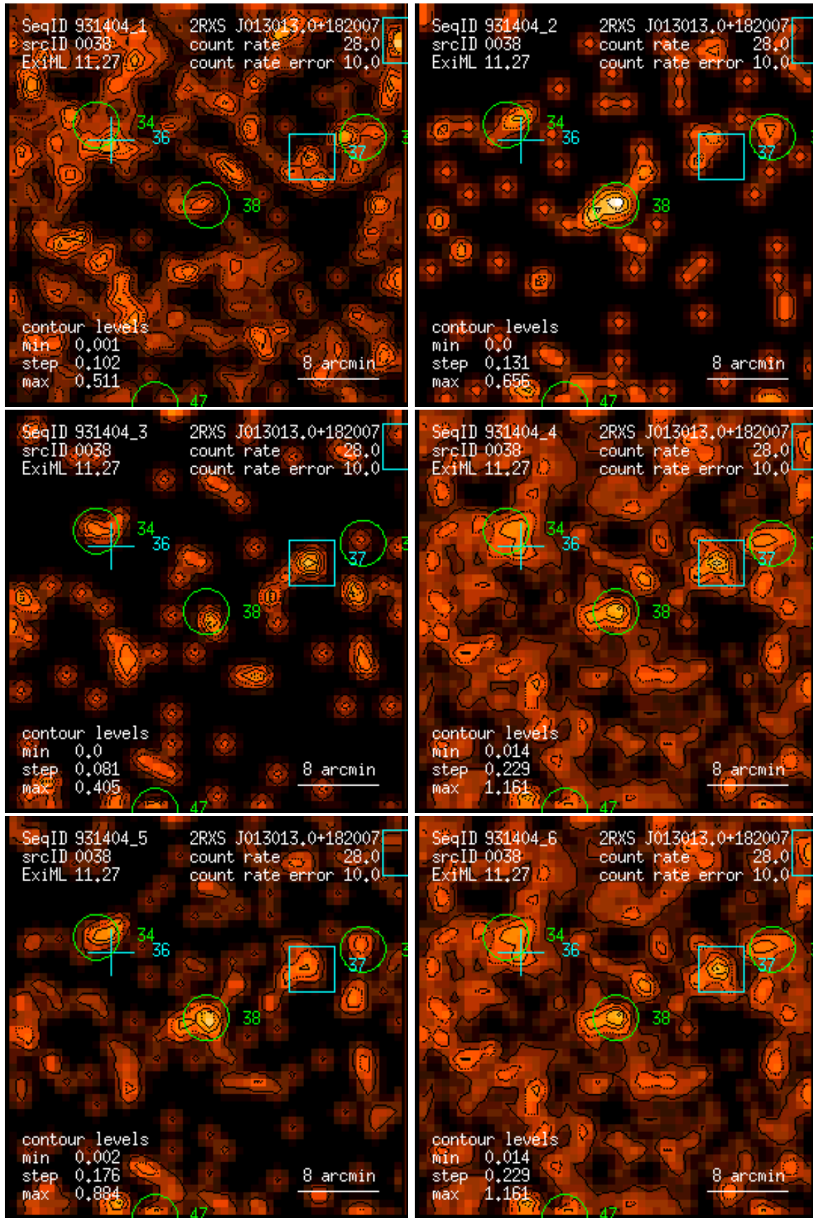
Figure 38: RASS 931404: detection 0038: band rate images, Gaussian filter: (1) PSPC channels 11 – 41, (2) 52 – 90, (3) 91 – 201, (4) 11 – 235, (5) 52 – 201, (6) 11 – 201. Broad band rates in counts/ks. Band rate contour levels in counts/ks/arcmin 2 .
