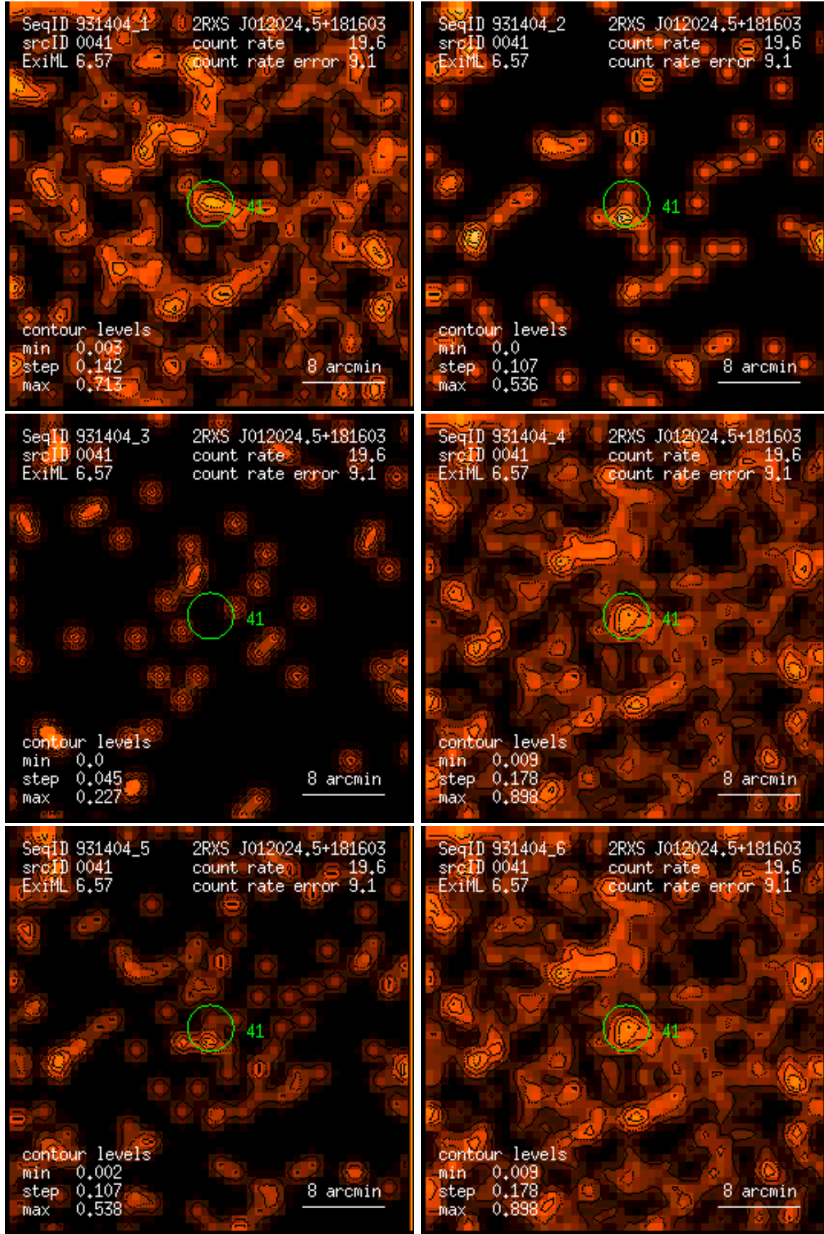
Figure 41: RASS 931404: detection 0041: band rate images, Gaussian filter: (1) PSPC channels 11 – 41, (2) 52 – 90, (3) 91 – 201, (4) 11 – 235, (5) 52 – 201, (6) 11 – 201. Broad band rates in counts/ks. Band rate contour levels in counts/ks/arcmin 2 .
