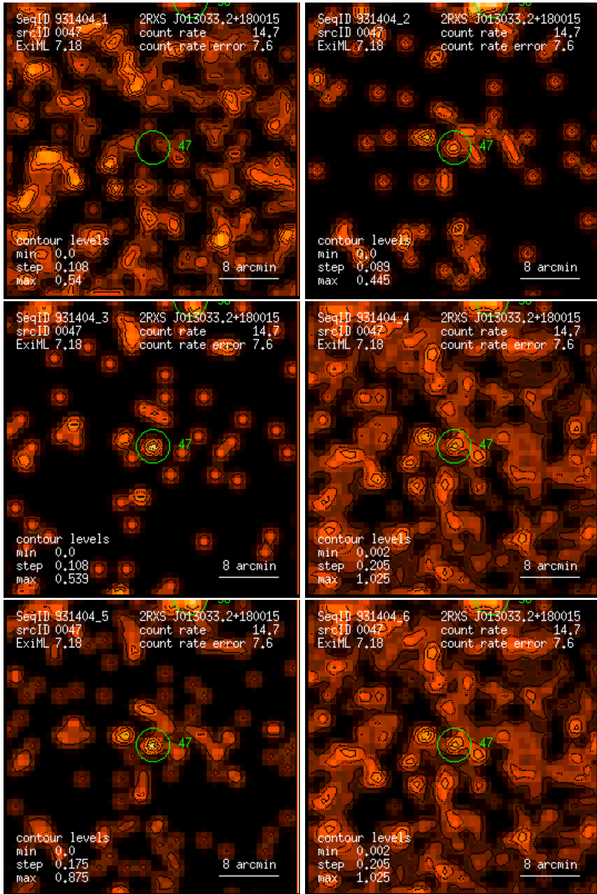
Figure 47: RASS 931404: detection 0047: band rate images, Gaussian filter: (1) PSPC channels 11 – 41, (2) 52 – 90, (3) 91 – 201, (4) 11 – 235, (5) 52 – 201, (6) 11 – 201. Broad band rates in counts/ks. Band rate contour levels in counts/ks/arcmin 2 .
