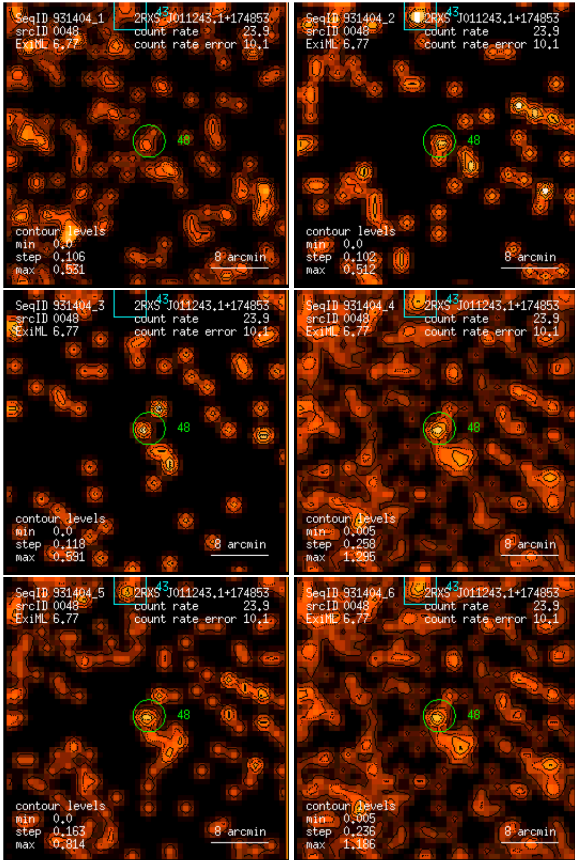
Figure 48: RASS 931404: detection 0048: band rate images, Gaussian filter: (1) PSPC channels 11 – 41, (2) 52 – 90, (3) 91 – 201, (4) 11 – 235, (5) 52 – 201, (6) 11 – 201. Broad band rates in counts/ks. Band rate contour levels in counts/ks/arcmin 2 .
