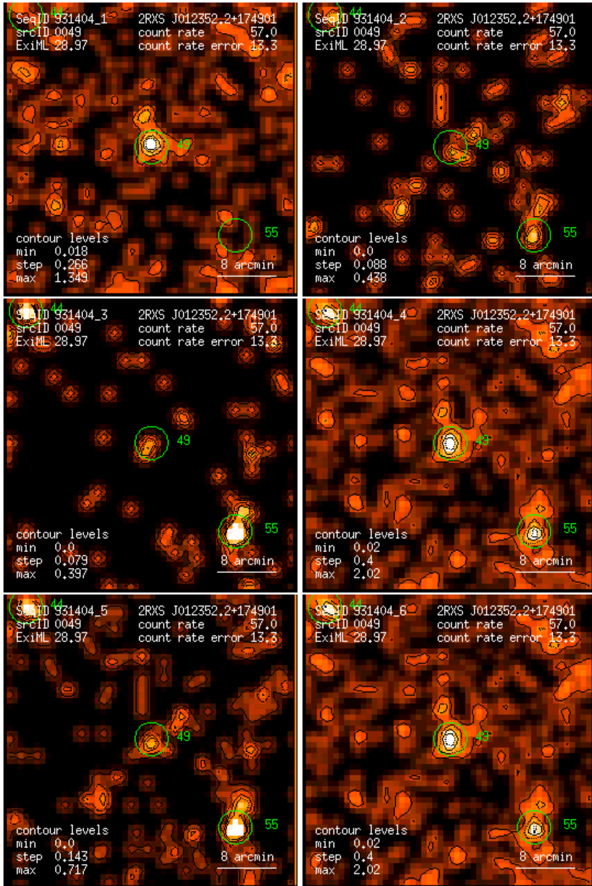
Figure 49: RASS 931404: detection 0049: band rate images, Gaussian filter: (1) PSPC channels 11 – 41, (2) 52 – 90, (3) 91 – 201, (4) 11 – 235, (5) 52 – 201, (6) 11 – 201. Broad band rates in counts/ks. Band rate contour levels in counts/ks/arcmin 2 .
