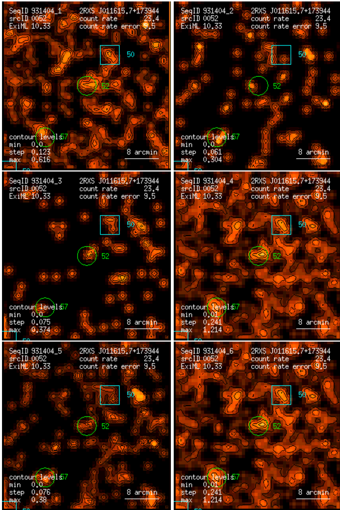
Figure 52: RASS 931404: detection 0052: band rate images, Gaussian filter: (1) PSPC channels 11 – 41, (2) 52 – 90, (3) 91 – 201, (4) 11 – 235, (5) 52 – 201, (6) 11 – 201. Broad band rates in counts/ks. Band rate contour levels in counts/ks/arcmin 2 .
