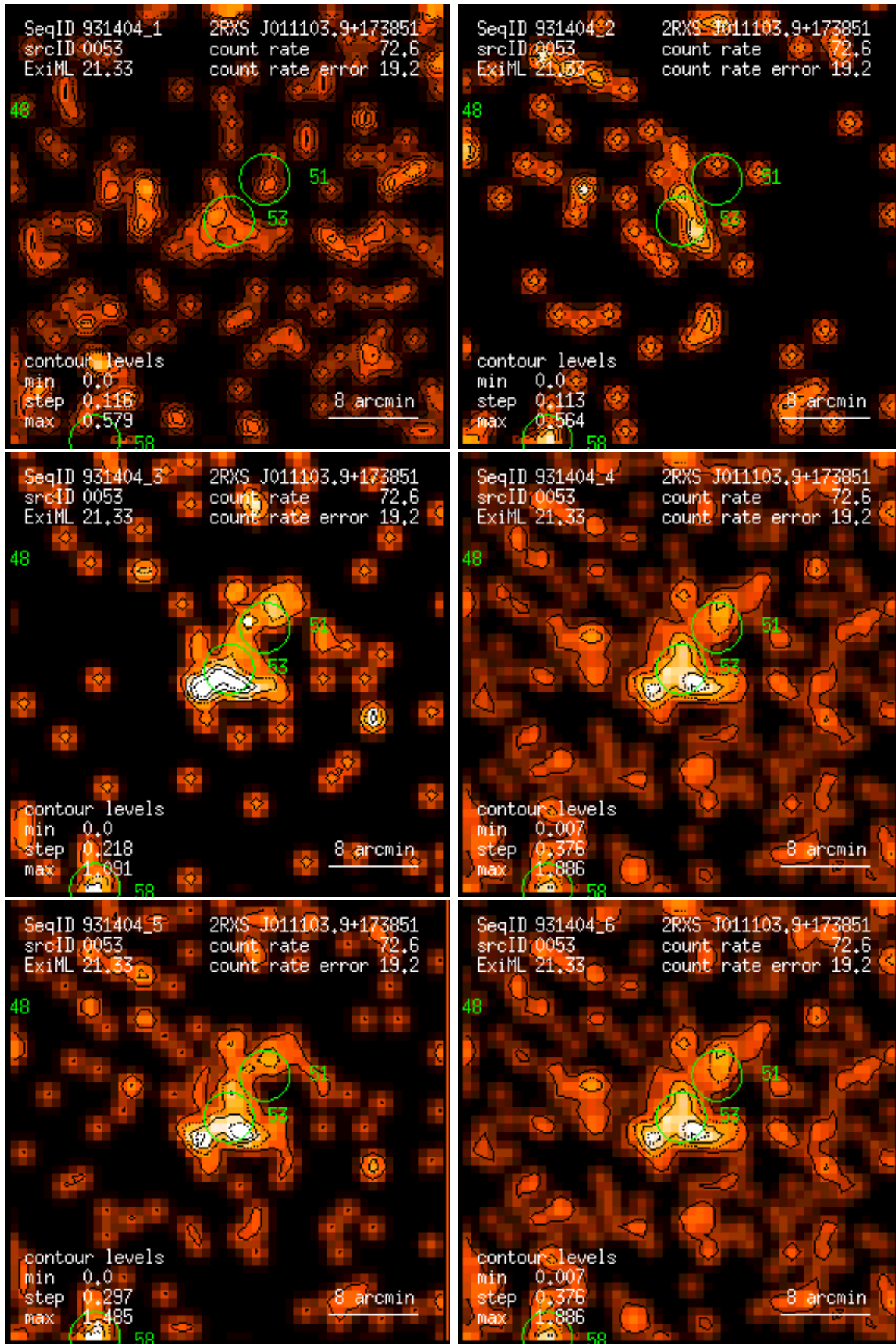
Figure 53: RASS 931404: detection 0053: band rate images, Gaussian filter: (1) PSPC channels 11 – 41, (2) 52 – 90, (3) 91 – 201, (4) 11 – 235, (5) 52 – 201, (6) 11 – 201. Broad band rates in counts/ks. Band rate contour levels in counts/ks/arcmin 2 .
