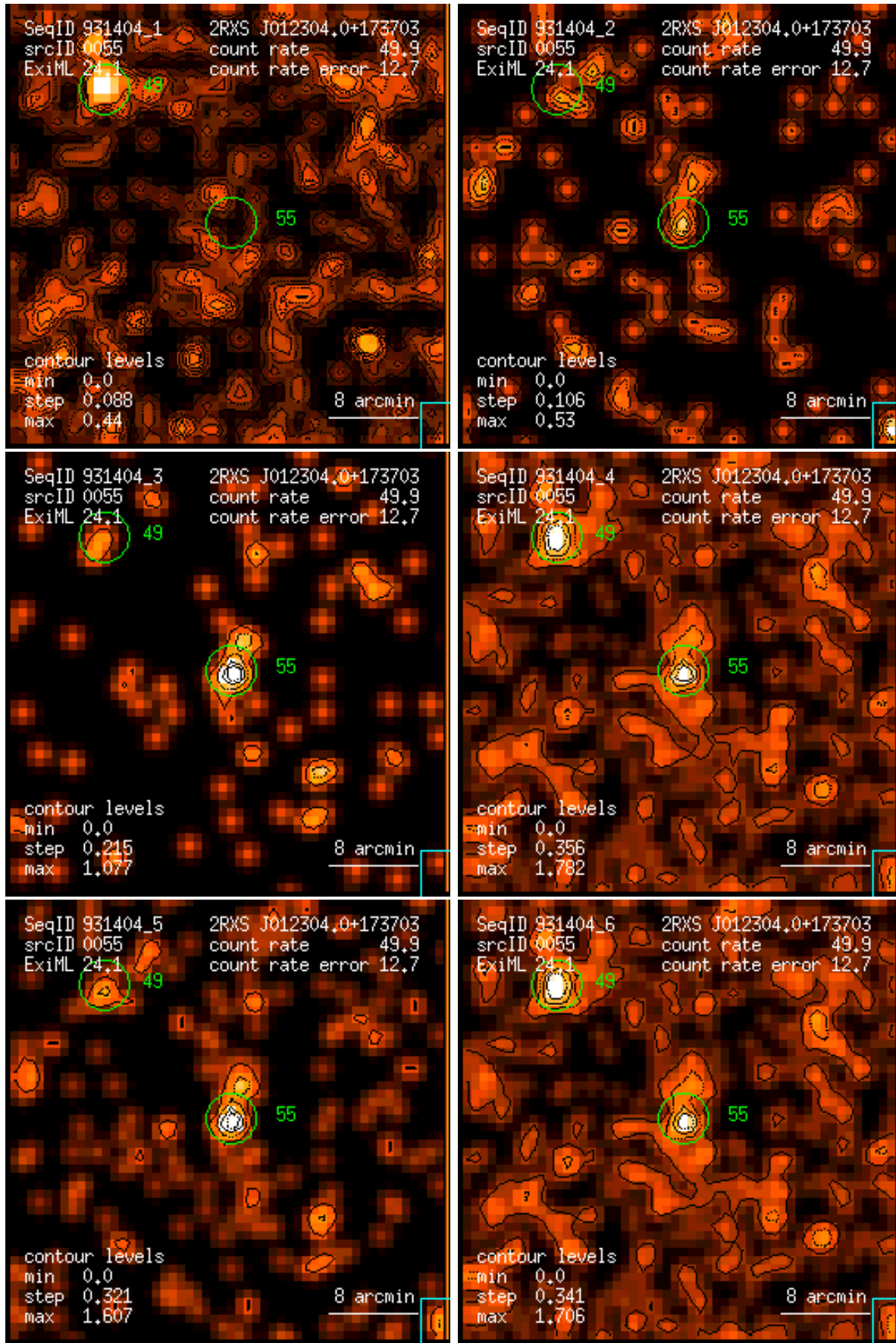
Figure 55: RASS 931404: detection 0055: band rate images, Gaussian filter: (1) PSPC channels 11 – 41, (2) 52 – 90, (3) 91 – 201, (4) 11 – 235, (5) 52 – 201, (6) 11 – 201. Broad band rates in counts/ks. Band rate contour levels in counts/ks/arcmin 2 .
