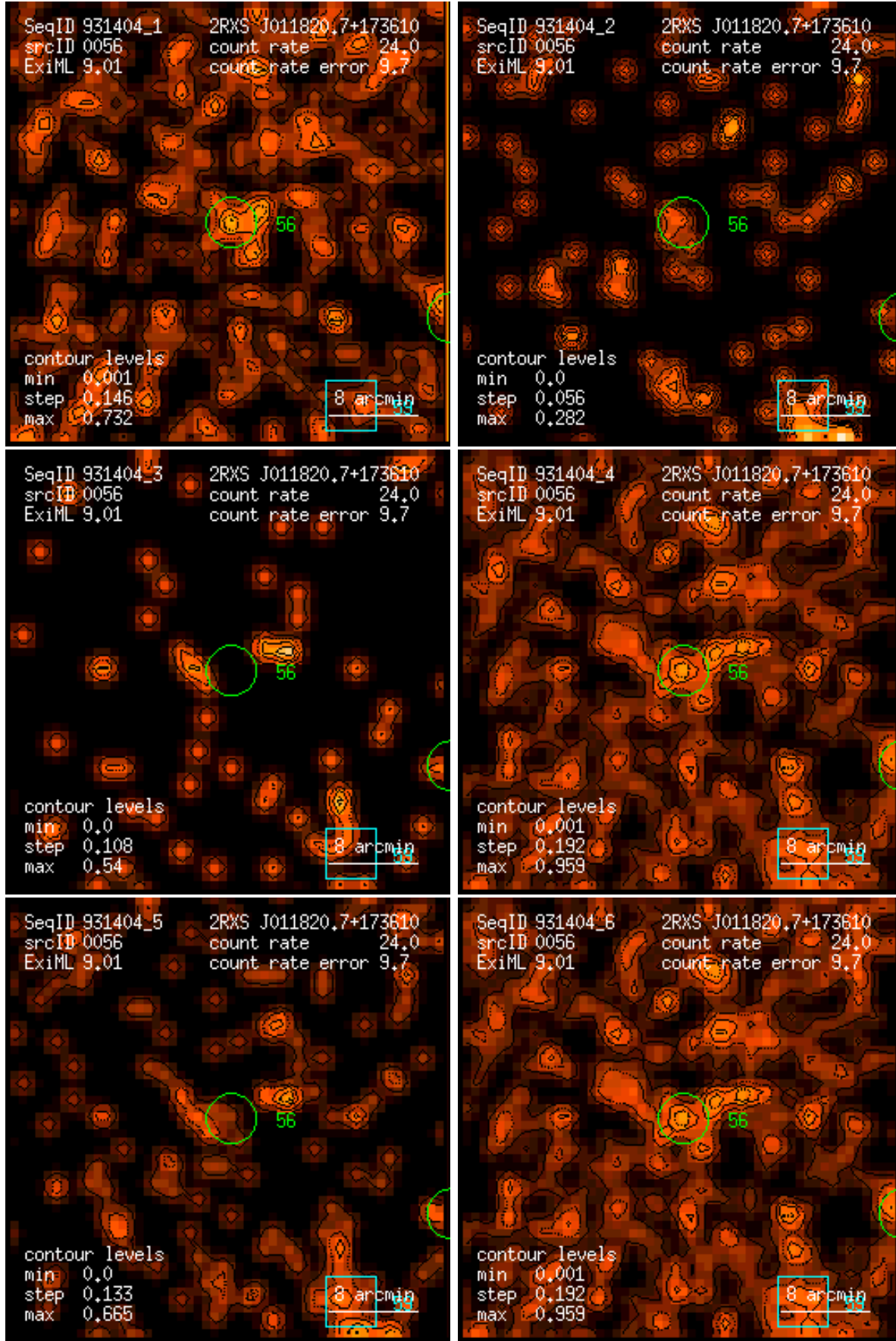
Figure 56: RASS 931404: detection 0056: band rate images, Gaussian filter: (1) PSPC channels 11 – 41, (2) 52 – 90, (3) 91 – 201, (4) 11 – 235, (5) 52 – 201, (6) 11 – 201. Broad band rates in counts/ks. Band rate contour levels in counts/ks/arcmin 2 .
