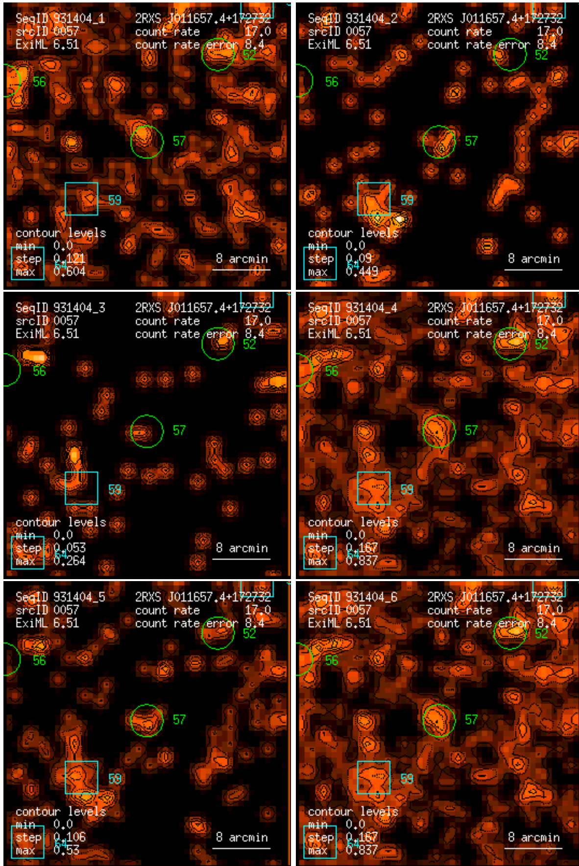
Figure 57: RASS 931404: detection 0057: band rate images, Gaussian filter: (1) PSPC channels 11 – 41, (2) 52 – 90, (3) 91 – 201, (4) 11 – 235, (5) 52 – 201, (6) 11 – 201. Broad band rates in counts/ks. Band rate contour levels in counts/ks/arcmin 2 .
