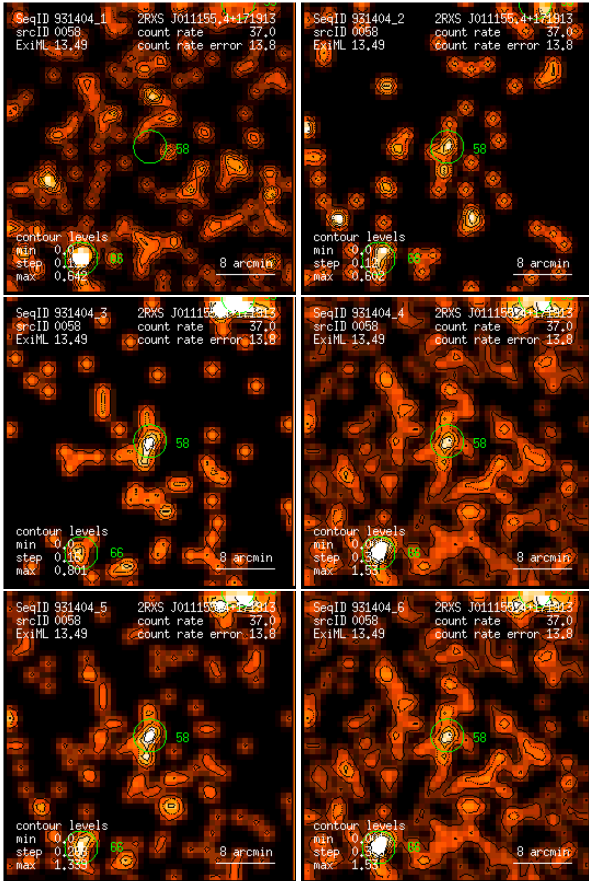
Figure 58: RASS 931404: detection 0058: band rate images, Gaussian filter: (1) PSPC channels 11 – 41, (2) 52 – 90, (3) 91 – 201, (4) 11 – 235, (5) 52 – 201, (6) 11 – 201. Broad band rates in counts/ks. Band rate contour levels in counts/ks/arcmin 2 .
