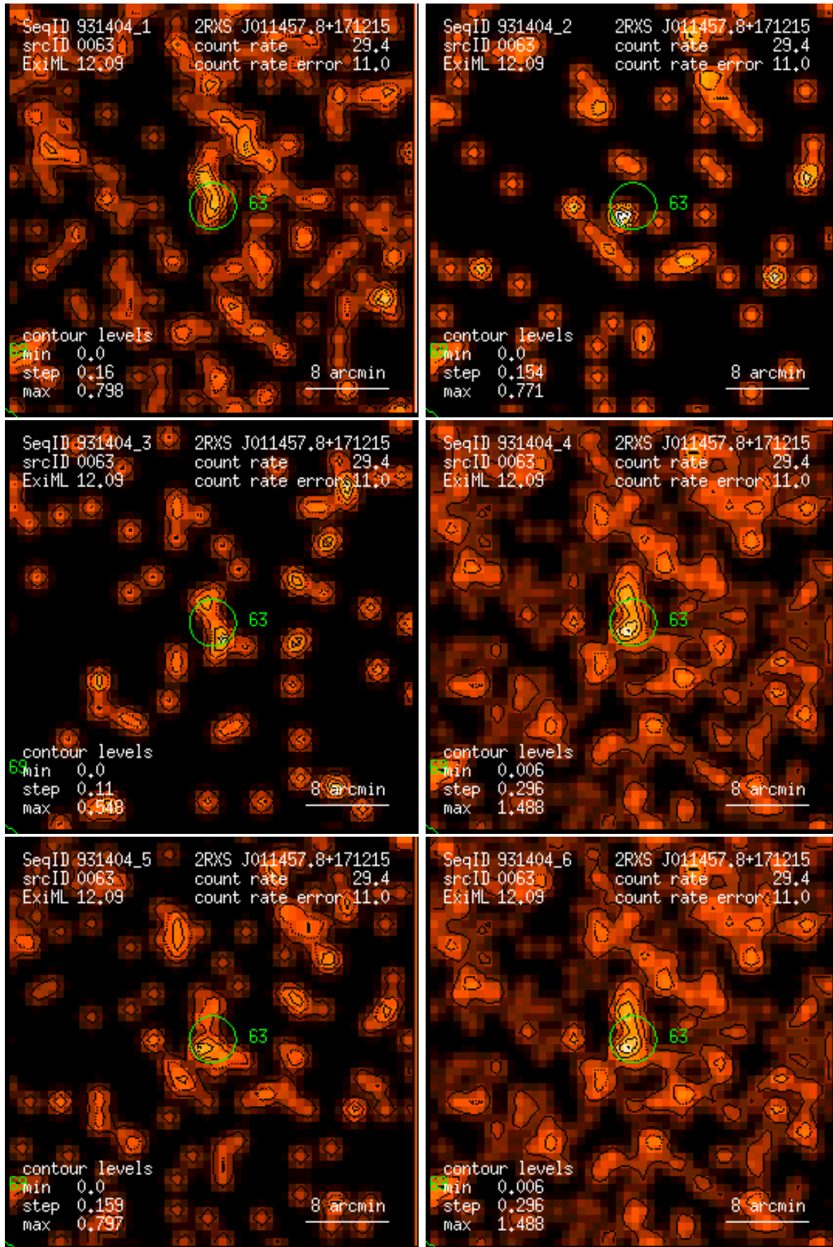
Figure 63: RASS 931404: detection 0063: band rate images, Gaussian filter: (1) PSPC channels 11 – 41, (2) 52 – 90, (3) 91 – 201, (4) 11 – 235, (5) 52 – 201, (6) 11 – 201. Broad band rates in counts/ks. Band rate contour levels in counts/ks/arcmin 2 .
