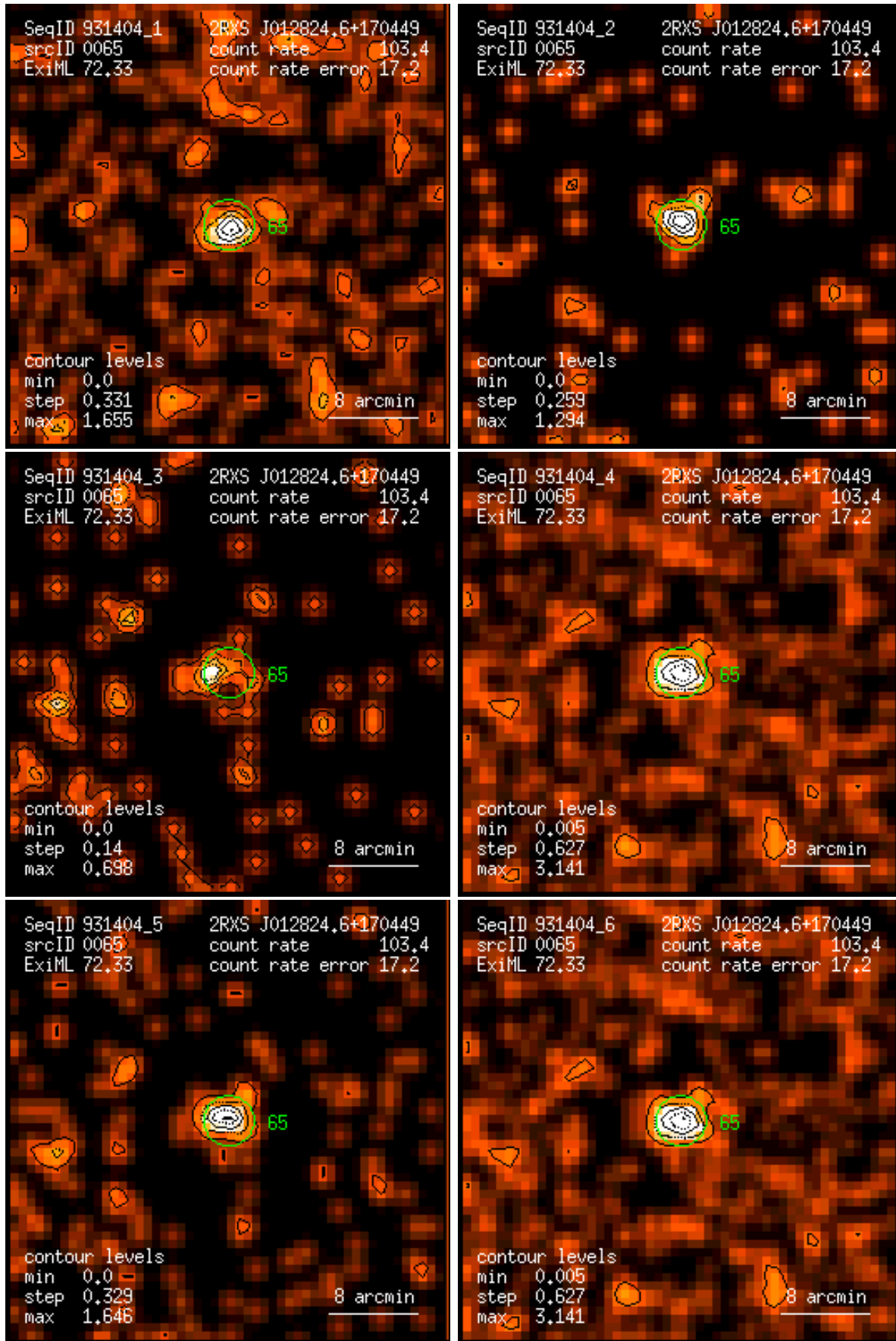
Figure 65: RASS 931404: detection 0065: band rate images, Gaussian filter: (1) PSPC channels 11 – 41, (2) 52 – 90, (3) 91 – 201, (4) 11 – 235, (5) 52 – 201, (6) 11 – 201. Broad band rates in counts/ks. Band rate contour levels in counts/ks/arcmin 2 .
