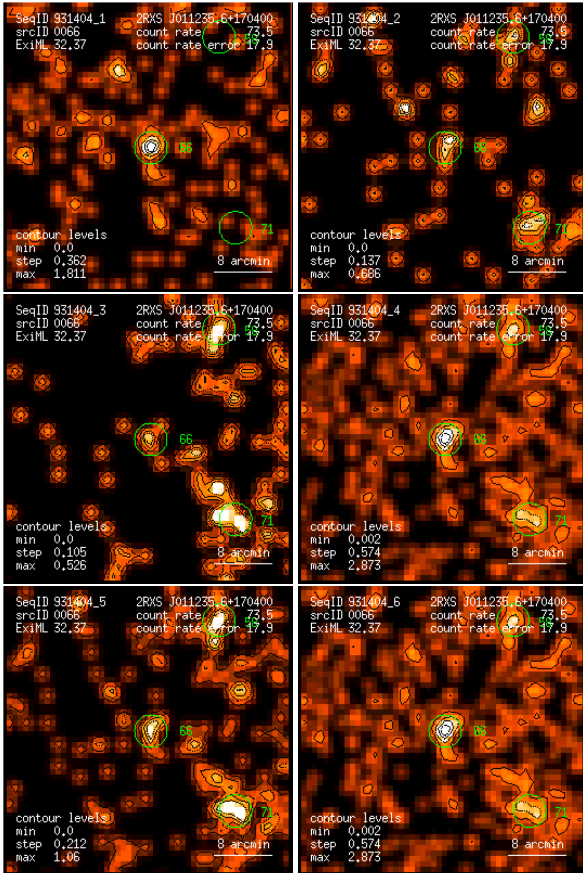
Figure 66: RASS 931404: detection 0066: band rate images, Gaussian filter: (1) PSPC channels 11 – 41, (2) 52 – 90, (3) 91 – 201, (4) 11 – 235, (5) 52 – 201, (6) 11 – 201. Broad band rates in counts/ks. Band rate contour levels in counts/ks/arcmin 2 .
