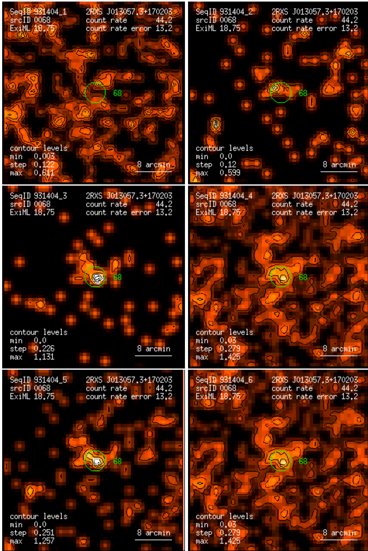
Figure 68: RASS 931404: detection 0068: band rate images, Gaussian filter: (1) PSPC channels 11 – 41, (2) 52 – 90, (3) 91 – 201, (4) 11 – 235, (5) 52 – 201, (6) 11 – 201. Broad band rates in counts/ks. Band rate contour levels in counts/ks/arcmin 2 .
