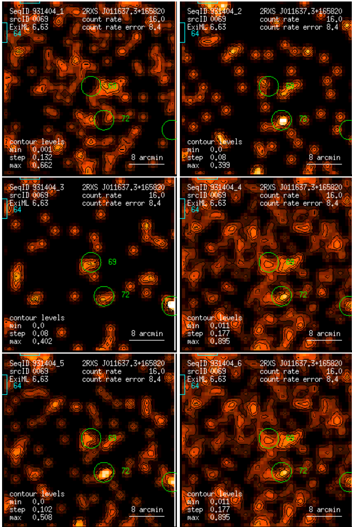
Figure 69: RASS 931404: detection 0069: band rate images, Gaussian filter: (1) PSPC channels 11 – 41, (2) 52 – 90, (3) 91 – 201, (4) 11 – 235, (5) 52 – 201, (6) 11 – 201. Broad band rates in counts/ks. Band rate contour levels in counts/ks/arcmin 2 .
