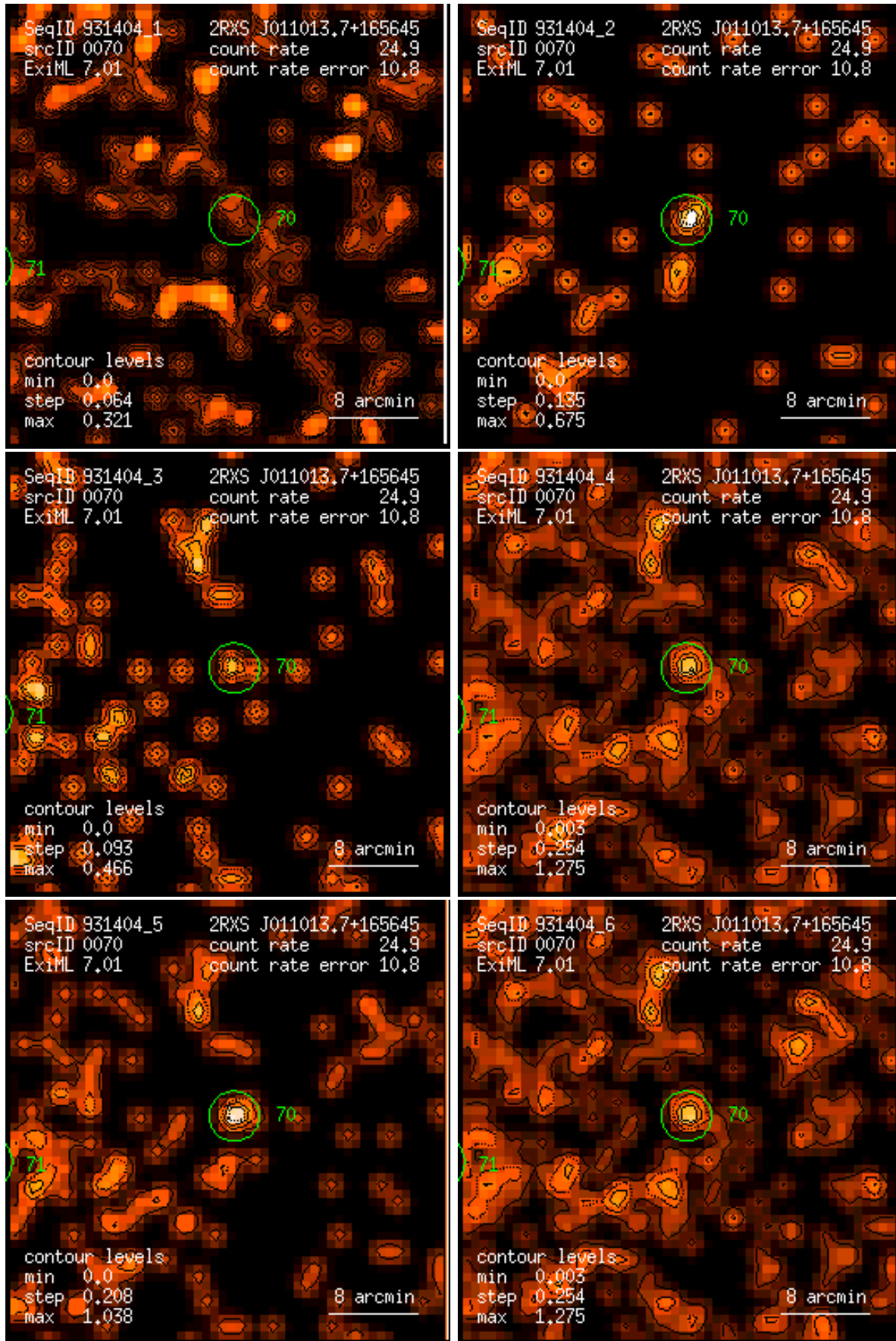
Figure 70: RASS 931404: detection 0070: band rate images, Gaussian filter: (1) PSPC channels 11 – 41, (2) 52 – 90, (3) 91 – 201, (4) 11 – 235, (5) 52 – 201, (6) 11 – 201. Broad band rates in counts/ks. Band rate contour levels in counts/ks/arcmin 2 .
