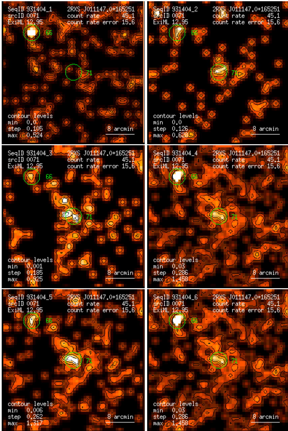
Figure 71: RASS 931404: detection 0071: band rate images, Gaussian filter: (1) PSPC channels 11 – 41, (2) 52 – 90, (3) 91 – 201, (4) 11 – 235, (5) 52 – 201, (6) 11 – 201. Broad band rates in counts/ks. Band rate contour levels in counts/ks/arcmin 2 .
