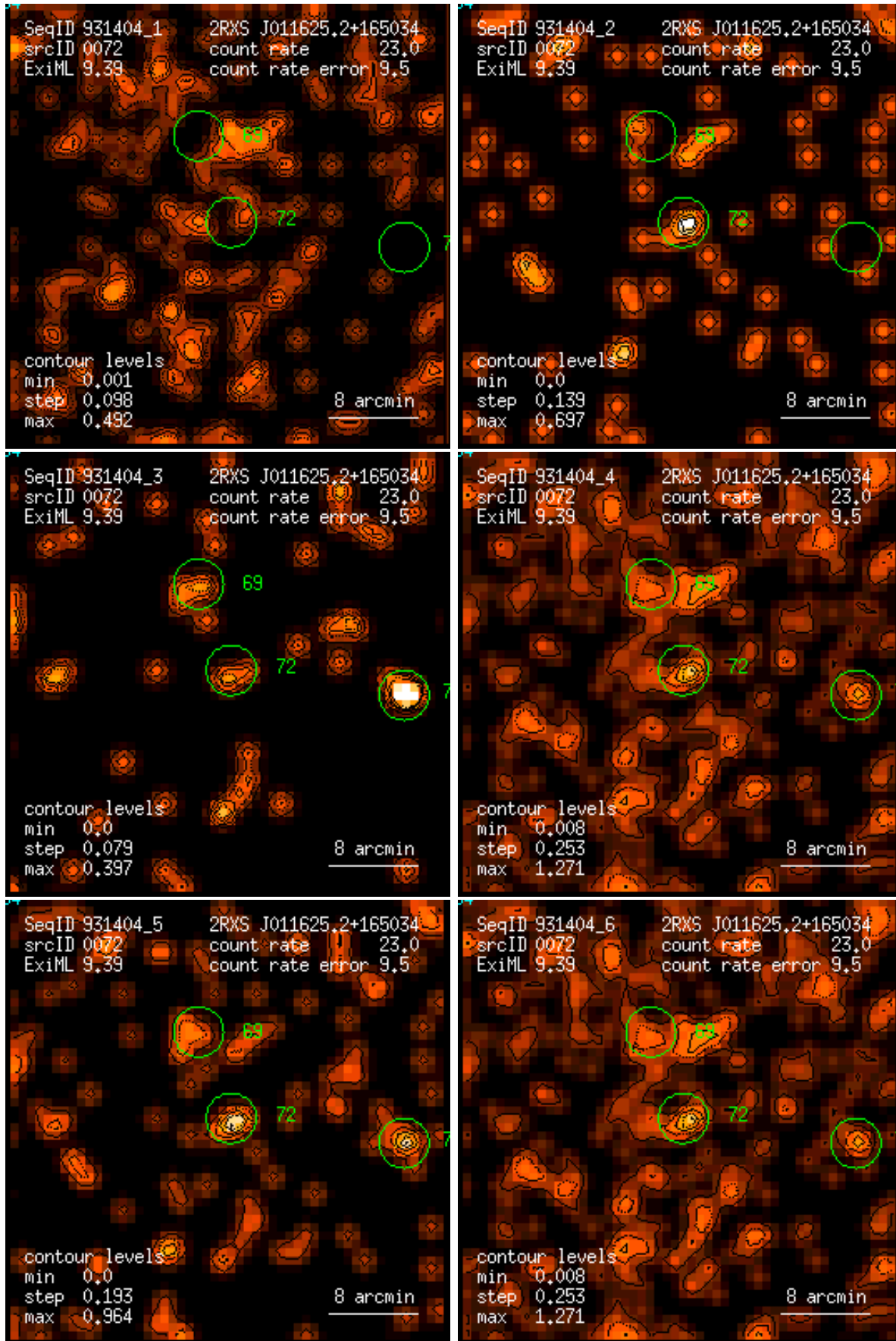
Figure 72: RASS 931404: detection 0072: band rate images, Gaussian filter: (1) PSPC channels 11 – 41, (2) 52 – 90, (3) 91 – 201, (4) 11 – 235, (5) 52 – 201, (6) 11 – 201. Broad band rates in counts/ks. Band rate contour levels in counts/ks/arcmin 2 .
