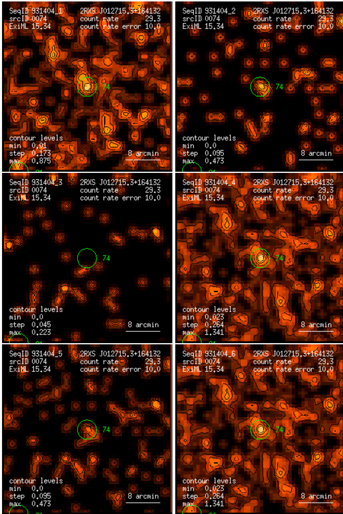
Figure 74: RASS 931404: detection 0074: band rate images, Gaussian filter: (1) PSPC channels 11 – 41, (2) 52 – 90, (3) 91 – 201, (4) 11 – 235, (5) 52 – 201, (6) 11 – 201. Broad band rates in counts/ks. Band rate contour levels in counts/ks/arcmin 2 .
