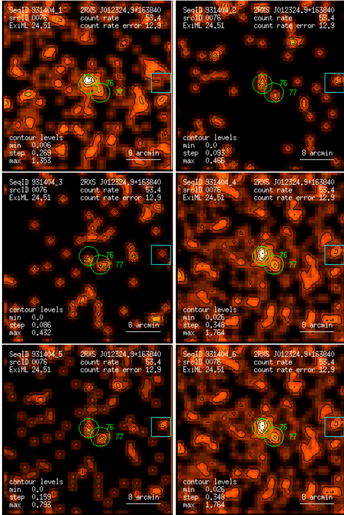
Figure 76: RASS 931404: detection 0076: band rate images, Gaussian filter: (1) PSPC channels 11 – 41, (2) 52 – 90, (3) 91 – 201, (4) 11 – 235, (5) 52 – 201, (6) 11 – 201. Broad band rates in counts/ks. Band rate contour levels in counts/ks/arcmin 2 .
