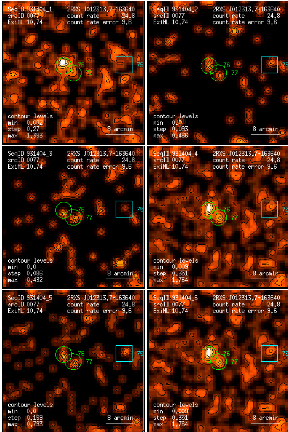
Figure 77: RASS 931404: detection 0077: band rate images, Gaussian filter: (1) PSPC channels 11 – 41, (2) 52 – 90, (3) 91 – 201, (4) 11 – 235, (5) 52 – 201, (6) 11 – 201. Broad band rates in counts/ks. Band rate contour levels in counts/ks/arcmin 2 .
