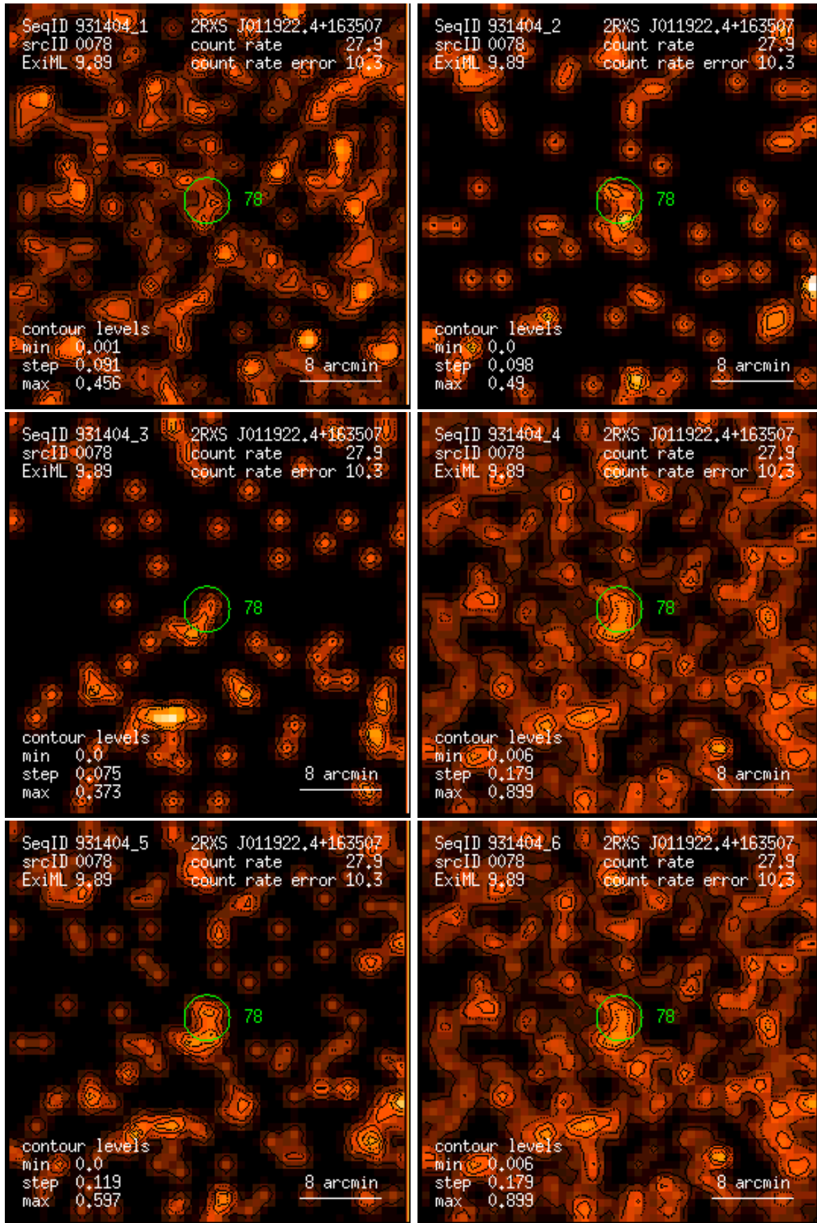
Figure 78: RASS 931404: detection 0078: band rate images, Gaussian filter: (1) PSPC channels 11 – 41, (2) 52 – 90, (3) 91 – 201, (4) 11 – 235, (5) 52 – 201, (6) 11 – 201. Broad band rates in counts/ks. Band rate contour levels in counts/ks/arcmin 2 .
