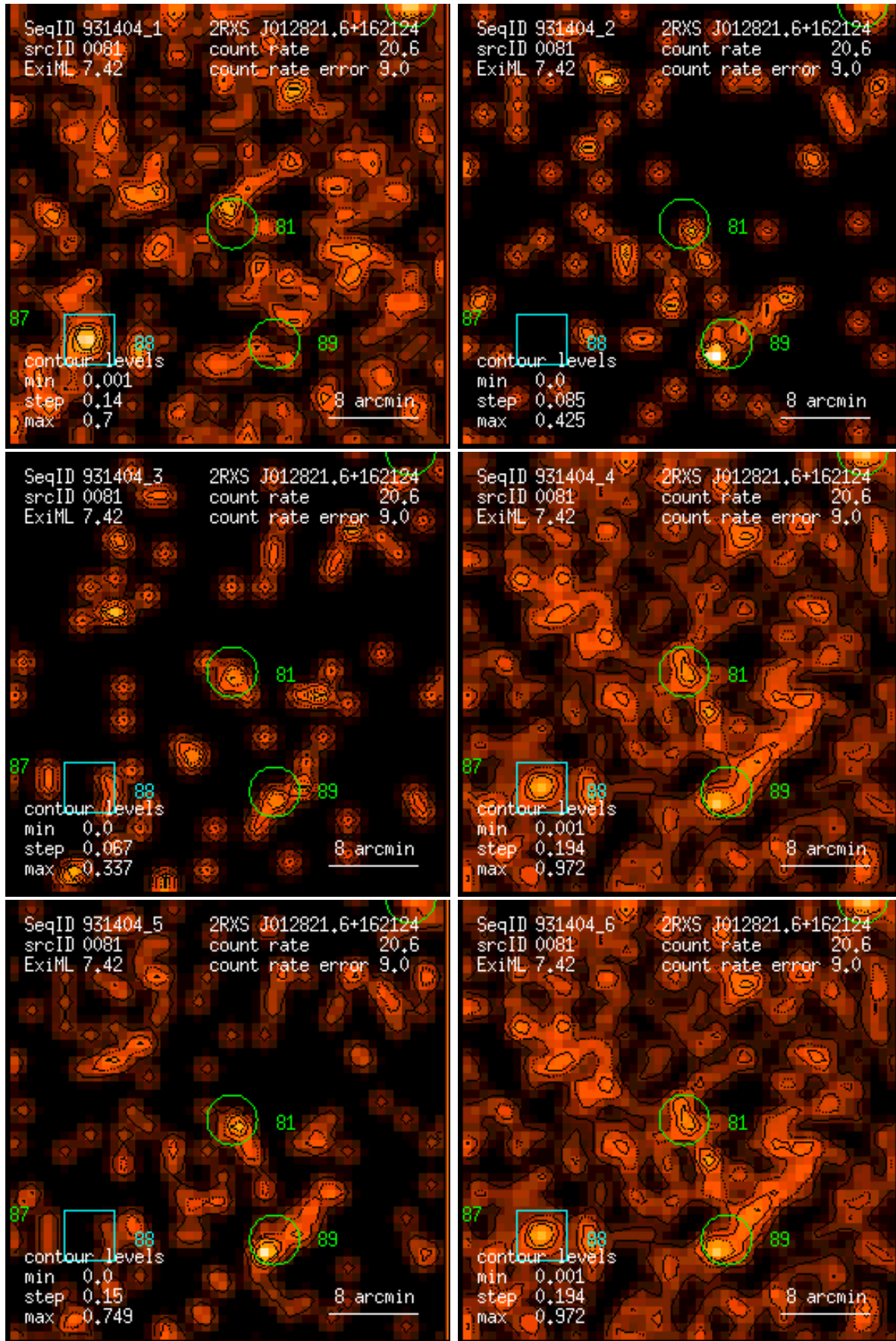
Figure 81: RASS 931404: detection 0081: band rate images, Gaussian filter: (1) PSPC channels 11 – 41, (2) 52 – 90, (3) 91 – 201, (4) 11 – 235, (5) 52 – 201, (6) 11 – 201. Broad band rates in counts/ks. Band rate contour levels in counts/ks/arcmin 2 .
