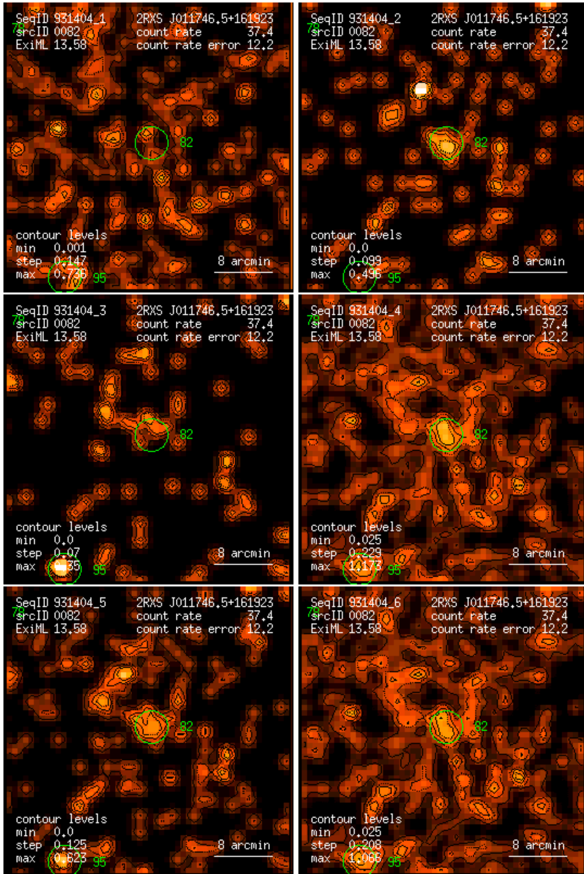
Figure 82: RASS 931404: detection 0082: band rate images, Gaussian filter: (1) PSPC channels 11 – 41, (2) 52 – 90, (3) 91 – 201, (4) 11 – 235, (5) 52 – 201, (6) 11 – 201. Broad band rates in counts/ks. Band rate contour levels in counts/ks/arcmin 2 .
