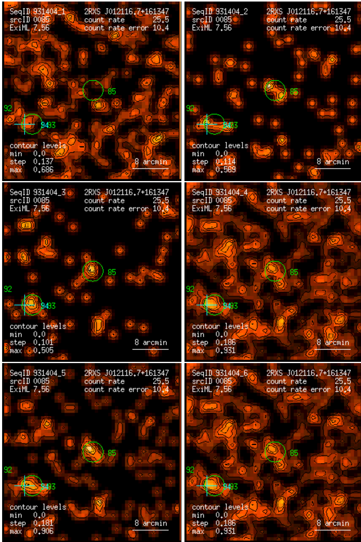
Figure 85: RASS 931404: detection 0085: band rate images, Gaussian filter: (1) PSPC channels 11 – 41, (2) 52 – 90, (3) 91 – 201, (4) 11 – 235, (5) 52 – 201, (6) 11 – 201. Broad band rates in counts/ks. Band rate contour levels in counts/ks/arcmin 2 .
