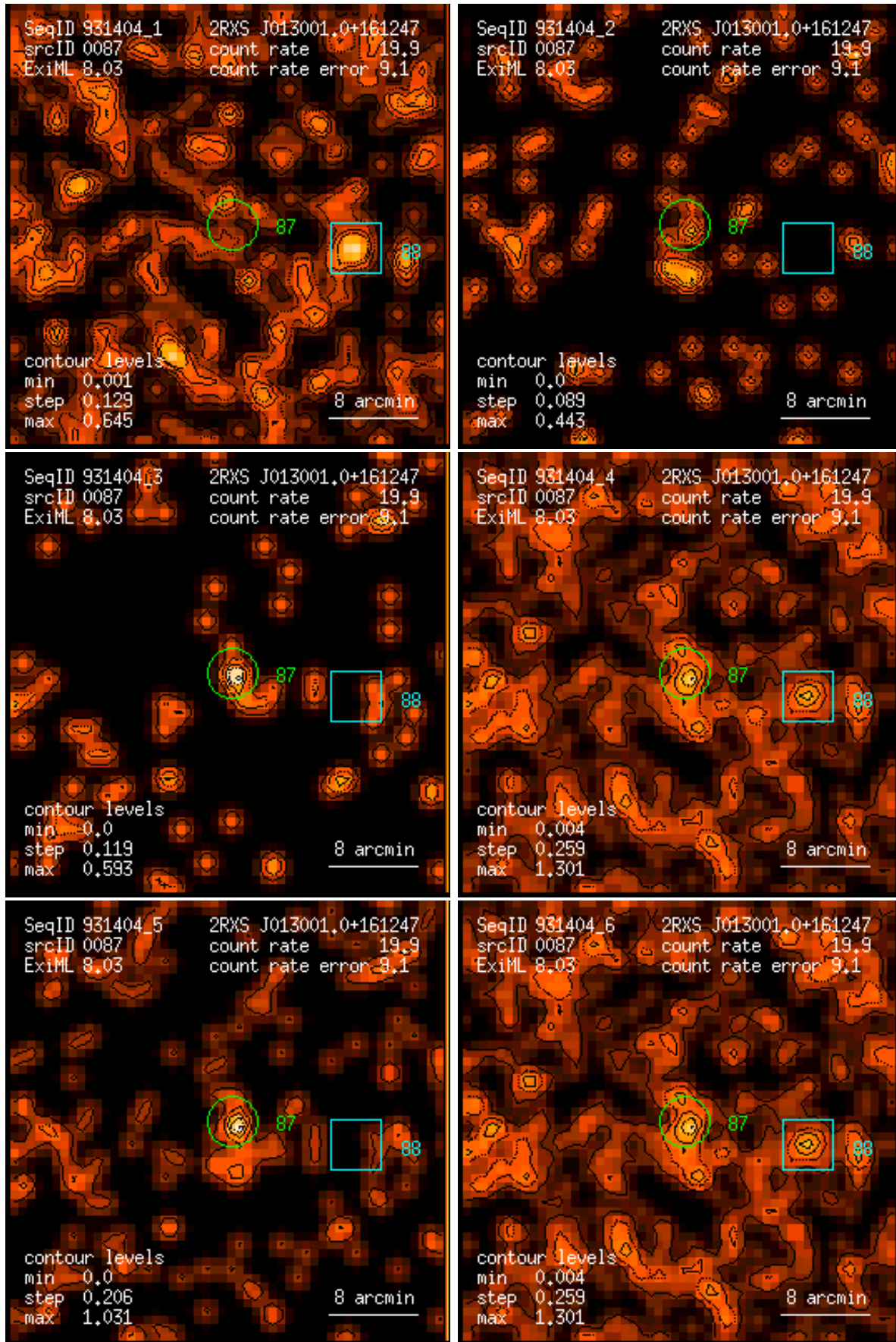
Figure 87: RASS 931404: detection 0087: band rate images, Gaussian filter: (1) PSPC channels 11 – 41, (2) 52 – 90, (3) 91 – 201, (4) 11 – 235, (5) 52 – 201, (6) 11 – 201. Broad band rates in counts/ks. Band rate contour levels in counts/ks/arcmin 2 .
