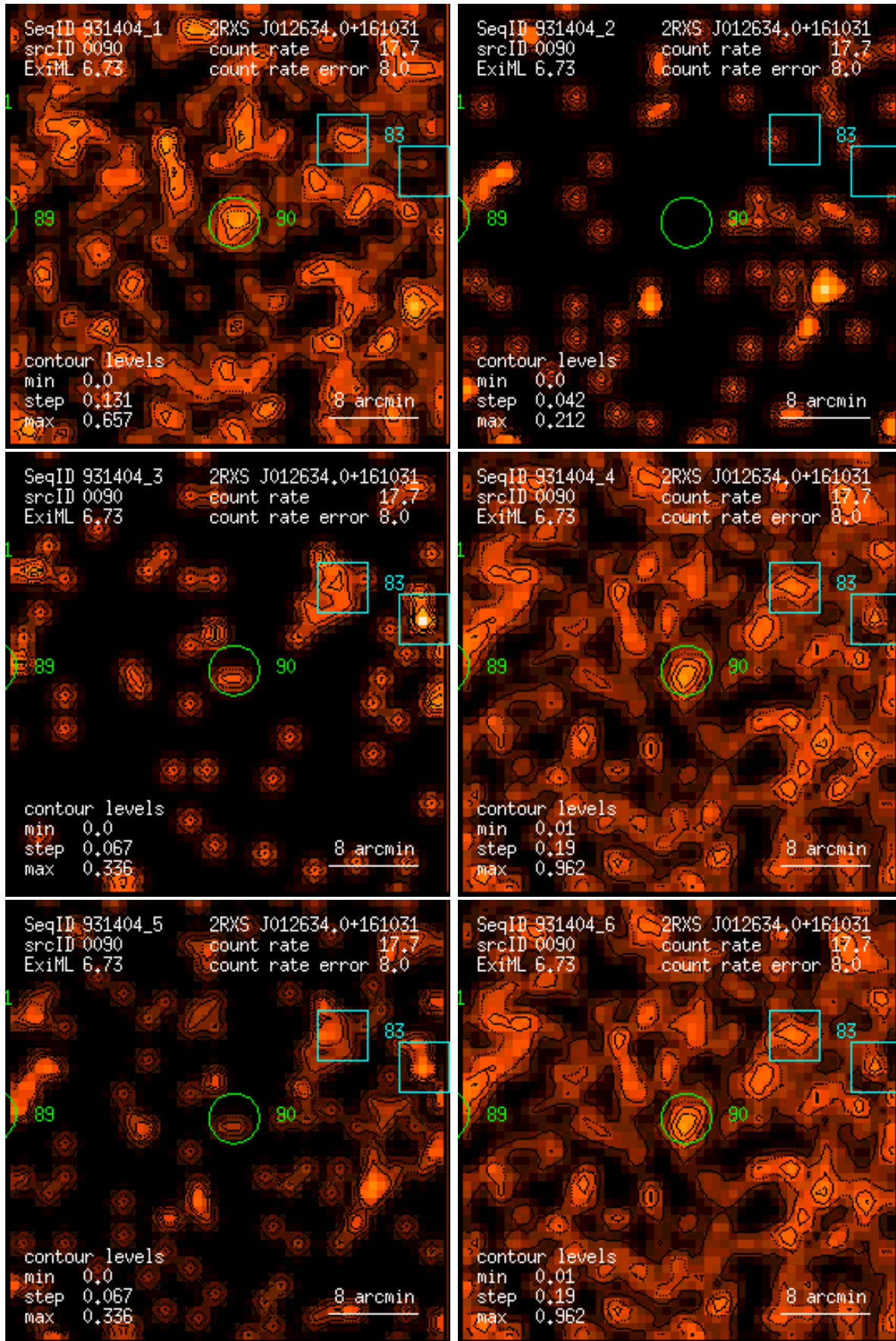
Figure 90: RASS 931404: detection 0090: band rate images, Gaussian filter: (1) PSPC channels 11 – 41, (2) 52 – 90, (3) 91 – 201, (4) 11 – 235, (5) 52 – 201, (6) 11 – 201. Broad band rates in counts/ks. Band rate contour levels in counts/ks/arcmin 2 .
