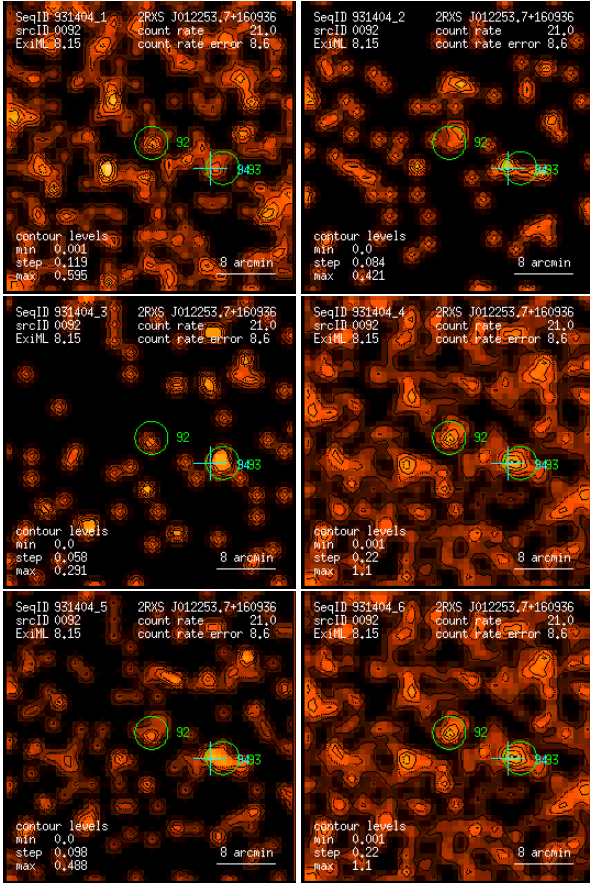
Figure 92: RASS 931404: detection 0092: band rate images, Gaussian filter: (1) PSPC channels 11 – 41, (2) 52 – 90, (3) 91 – 201, (4) 11 – 235, (5) 52 – 201, (6) 11 – 201. Broad band rates in counts/ks. Band rate contour levels in counts/ks/arcmin 2 .
