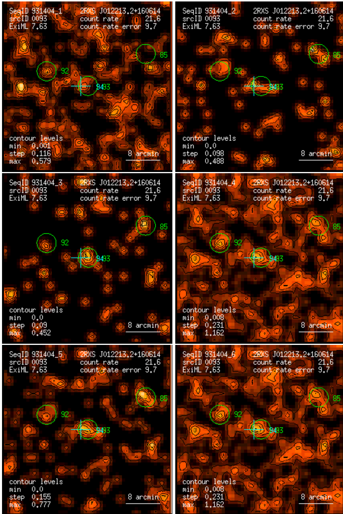
Figure 93: RASS 931404: detection 0093: band rate images, Gaussian filter: (1) PSPC channels 11 – 41, (2) 52 – 90, (3) 91 – 201, (4) 11 – 235, (5) 52 – 201, (6) 11 – 201. Broad band rates in counts/ks. Band rate contour levels in counts/ks/arcmin 2 .
