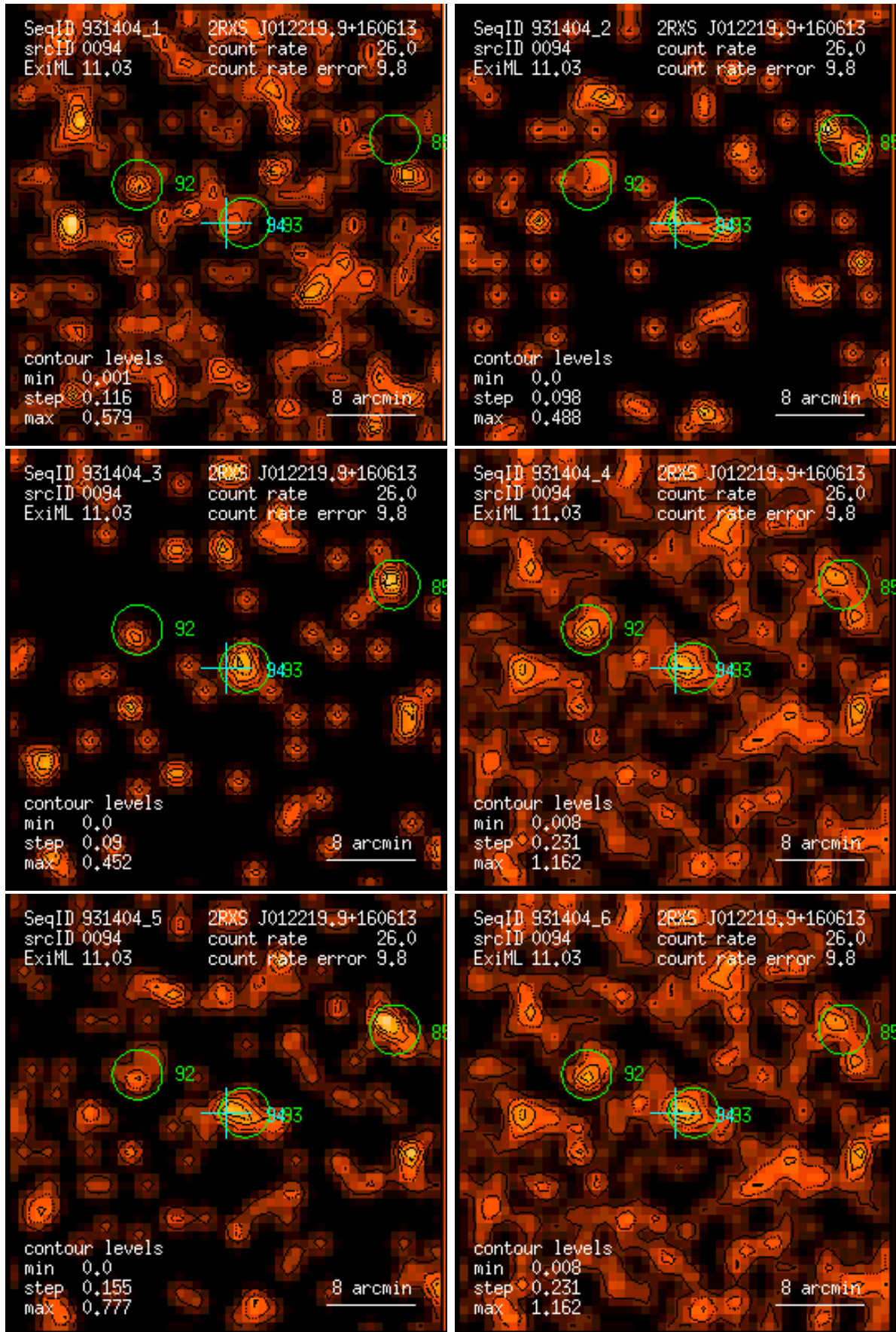
Figure 94: RASS 931404: detection 0094: band rate images, Gaussian filter: (1) PSPC channels 11 – 41, (2) 52 – 90, (3) 91 – 201, (4) 11 – 235, (5) 52 – 201, (6) 11 – 201. Broad band rates in counts/ks. Band rate contour levels in counts/ks/arcmin 2 .
