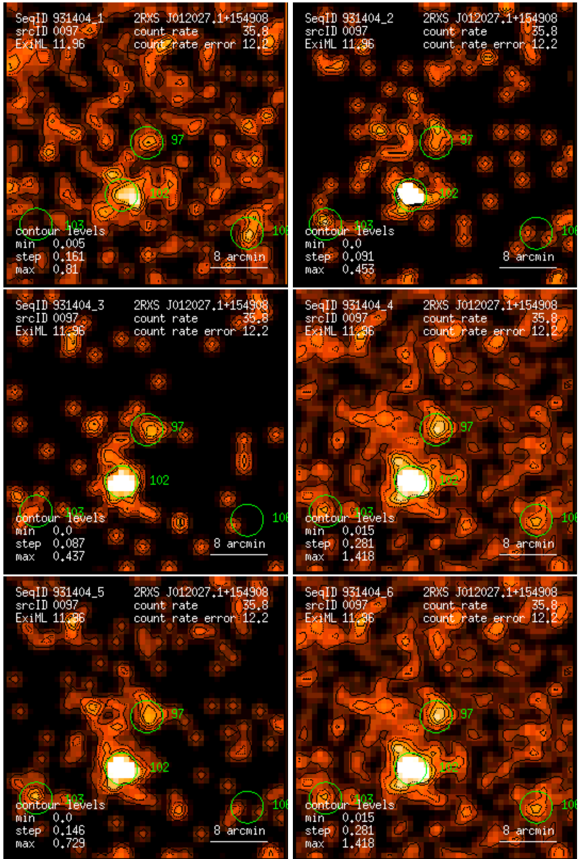
Figure 97: RASS 931404: detection 0097: band rate images, Gaussian filter: (1) PSPC channels 11 – 41, (2) 52 – 90, (3) 91 – 201, (4) 11 – 235, (5) 52 – 201, (6) 11 – 201. Broad band rates in counts/ks. Band rate contour levels in counts/ks/arcmin 2 .
