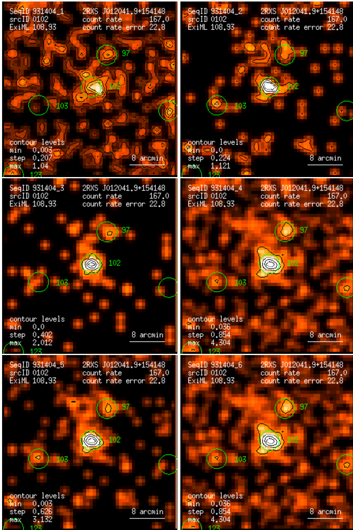
Figure 102: RASS 931404: detection 0102: band rate images, Gaussian filter: (1) PSPC channels 11 – 41, (2) 52 – 90, (3) 91 – 201, (4) 11 – 235, (5) 52 – 201, (6) 11 – 201. Broad band rates in counts/ks. Band rate contour levels in counts/ks/arcmin 2 .
