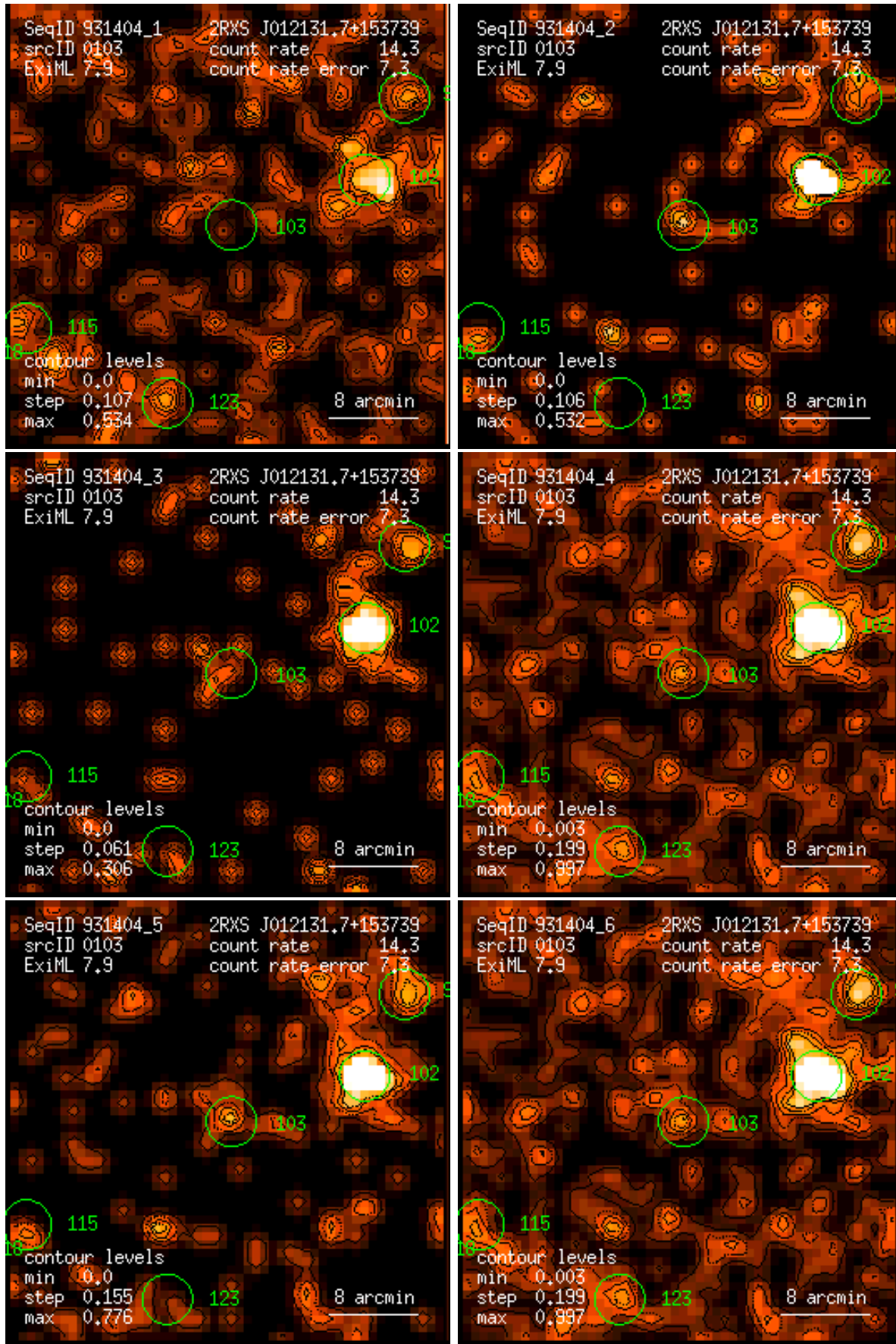
Figure 103: RASS 931404: detection 0103: band rate images, Gaussian filter: (1) PSPC channels 11 – 41, (2) 52 – 90, (3) 91 – 201, (4) 11 – 235, (5) 52 – 201, (6) 11 – 201. Broad band rates in counts/ks. Band rate contour levels in counts/ks/arcmin 2 .
