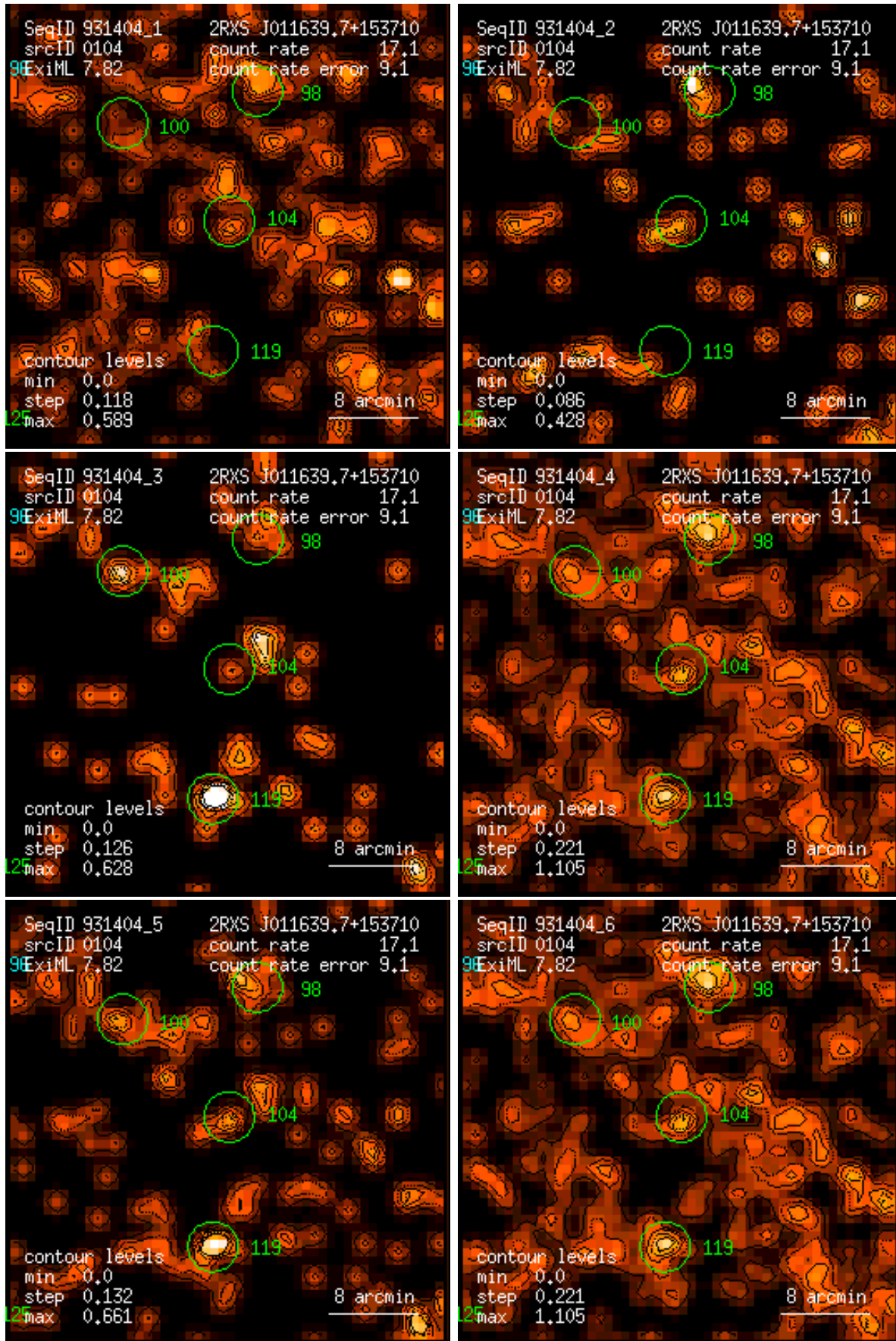
Figure 104: RASS 931404: detection 0104: band rate images, Gaussian filter: (1) PSPC channels 11 – 41, (2) 52 – 90, (3) 91 – 201, (4) 11 – 235, (5) 52 – 201, (6) 11 – 201. Broad band rates in counts/ks. Band rate contour levels in counts/ks/arcmin 2 .
