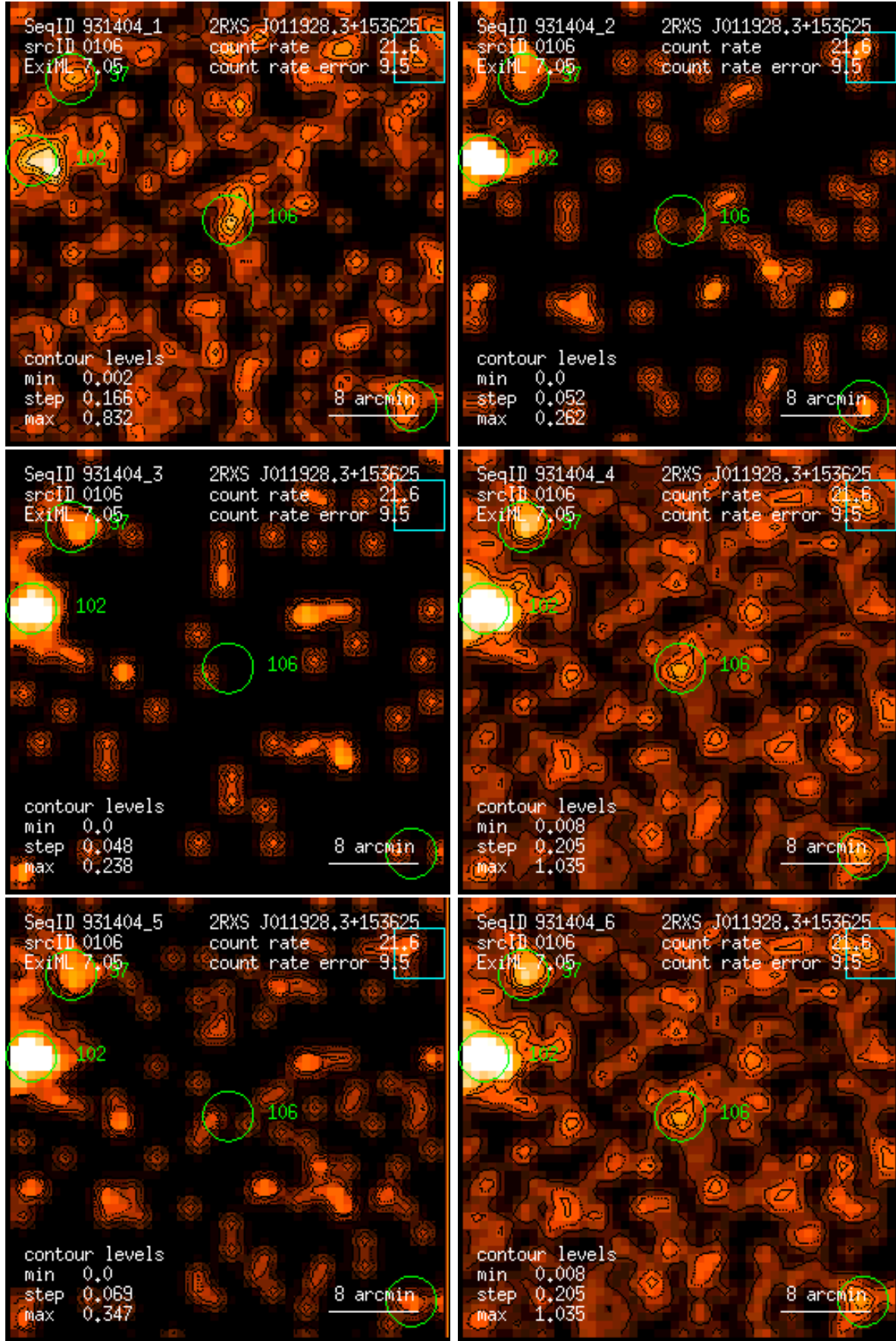
Figure 106: RASS 931404: detection 0106: band rate images, Gaussian filter: (1) PSPC channels 11 – 41, (2) 52 – 90, (3) 91 – 201, (4) 11 – 235, (5) 52 – 201, (6) 11 – 201. Broad band rates in counts/ks. Band rate contour levels in counts/ks/arcmin 2 .
