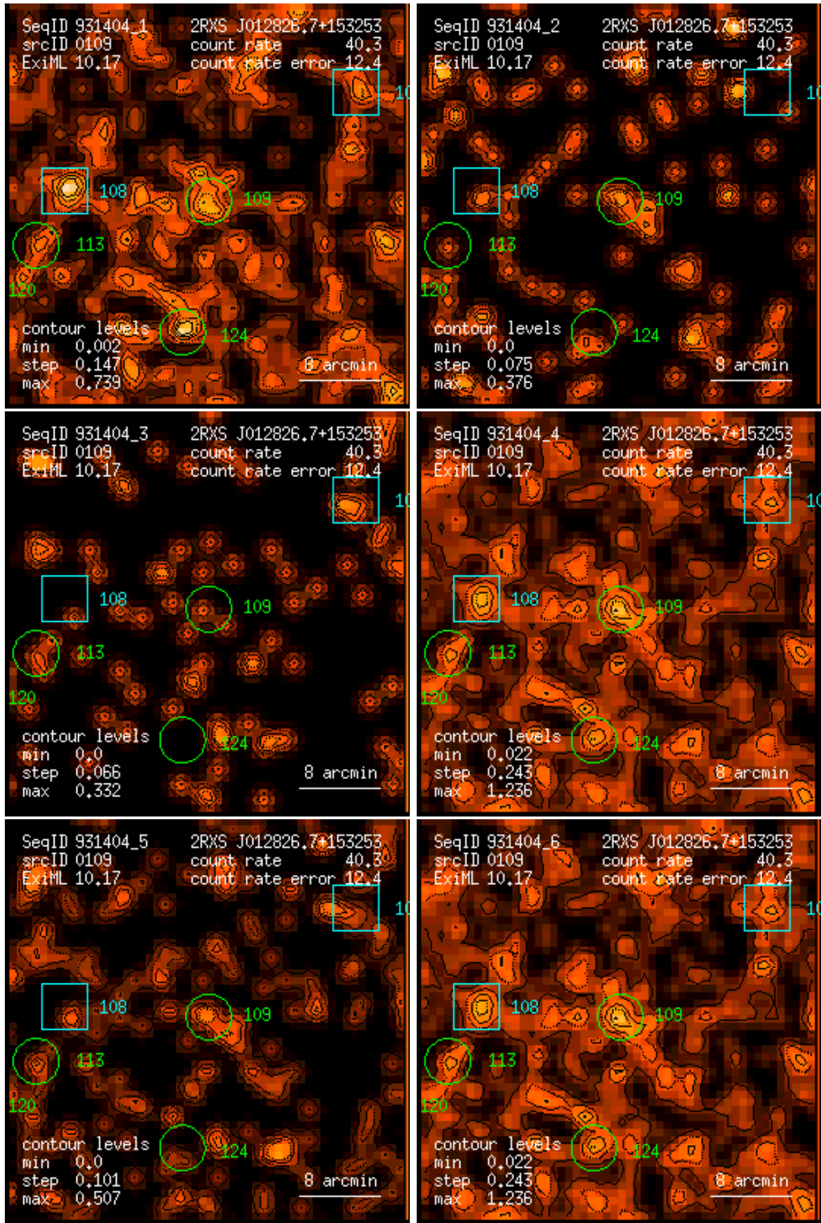
Figure 109: RASS 931404: detection 0109: band rate images, Gaussian filter: (1) PSPC channels 11 – 41, (2) 52 – 90, (3) 91 – 201, (4) 11 – 235, (5) 52 – 201, (6) 11 – 201. Broad band rates in counts/ks. Band rate contour levels in counts/ks/arcmin 2 .
