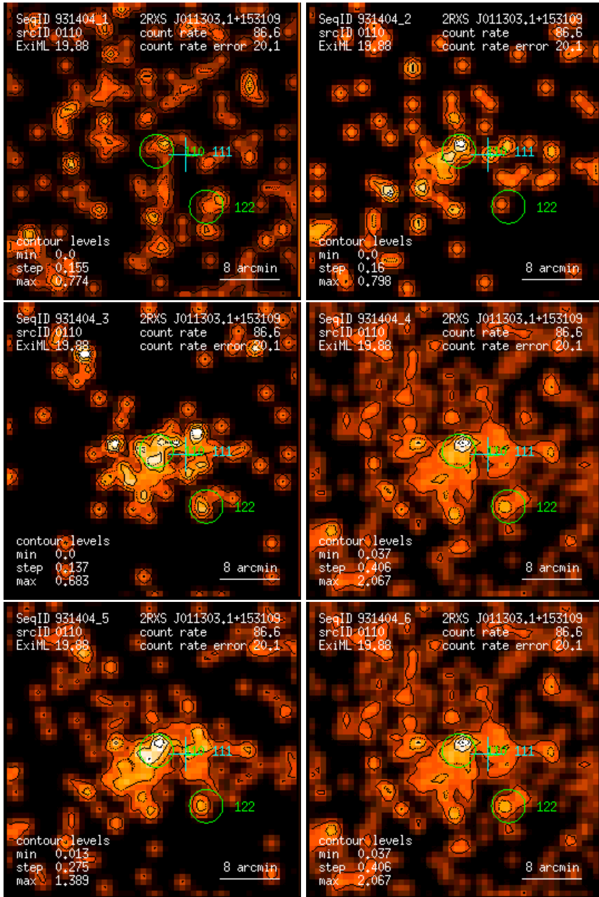
Figure 110: RASS 931404: detection 0110: band rate images, Gaussian filter: (1) PSPC channels 11 – 41, (2) 52 – 90, (3) 91 – 201, (4) 11 – 235, (5) 52 – 201, (6) 11 – 201. Broad band rates in counts/ks. Band rate contour levels in counts/ks/arcmin 2 .
