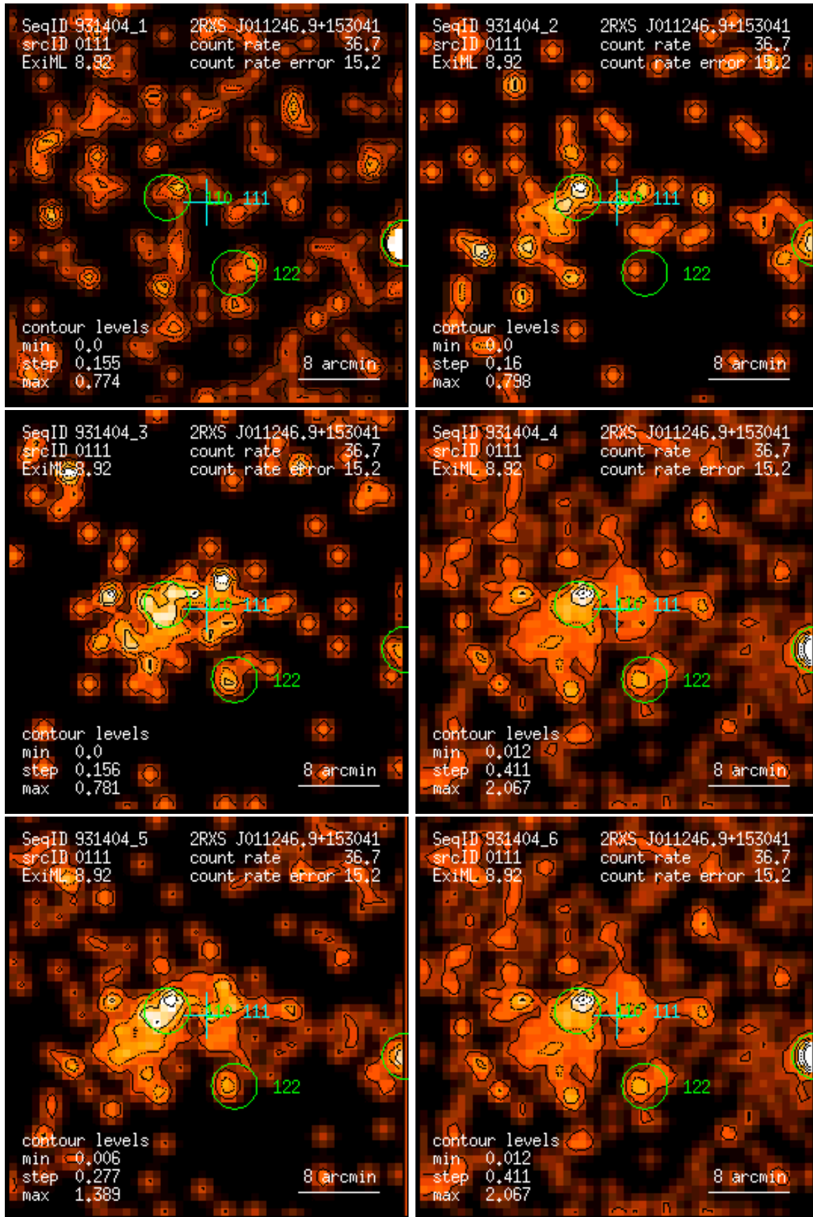
Figure 111: RASS 931404: detection 0111: band rate images, Gaussian filter: (1) PSPC channels 11 – 41, (2) 52 – 90, (3) 91 – 201, (4) 11 – 235, (5) 52 – 201, (6) 11 – 201. Broad band rates in counts/ks. Band rate contour levels in counts/ks/arcmin 2 .
