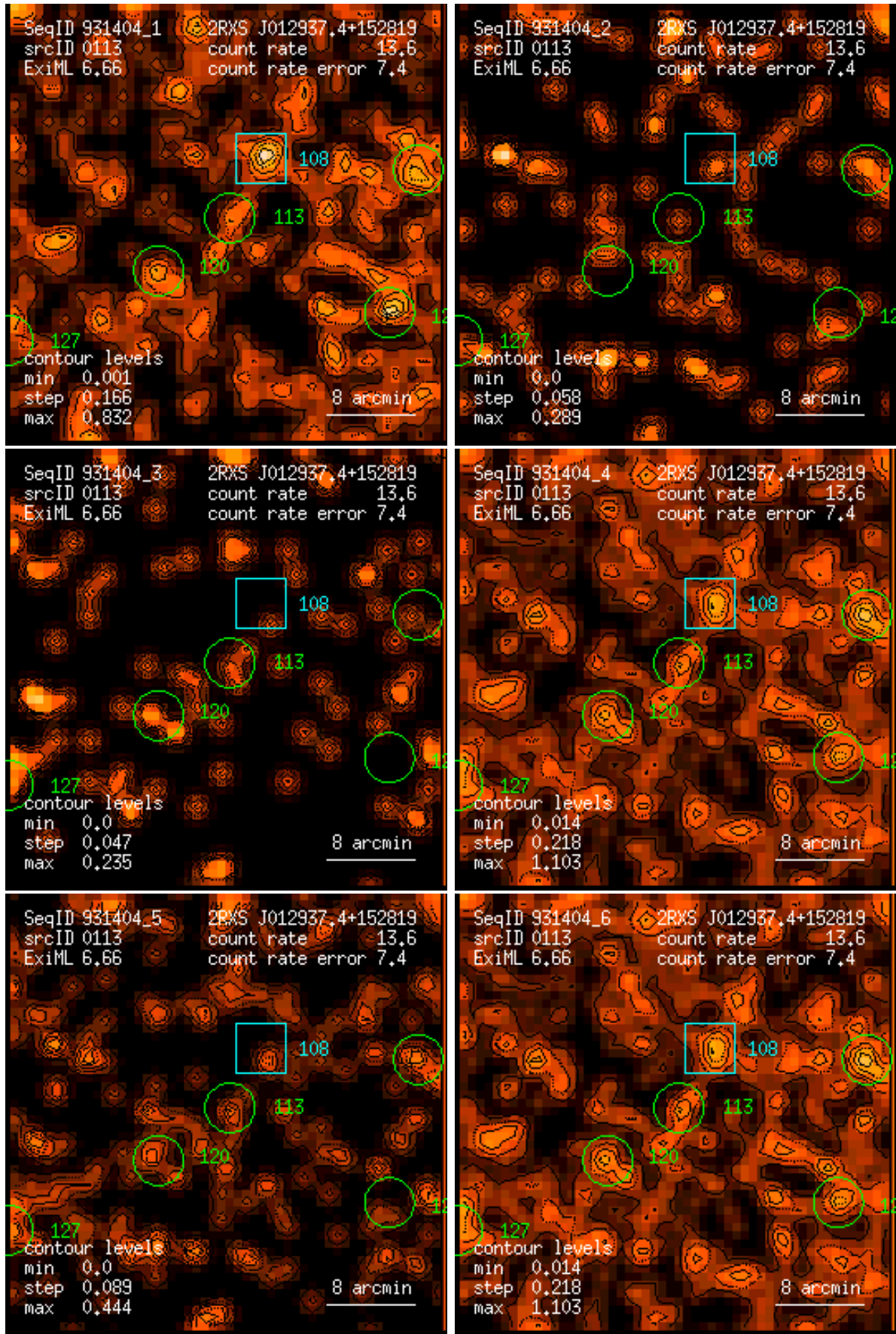
Figure 113: RASS 931404: detection 0113: band rate images, Gaussian filter: (1) PSPC channels 11 – 41, (2) 52 – 90, (3) 91 – 201, (4) 11 – 235, (5) 52 – 201, (6) 11 – 201. Broad band rates in counts/ks. Band rate contour levels in counts/ks/arcmin 2 .
