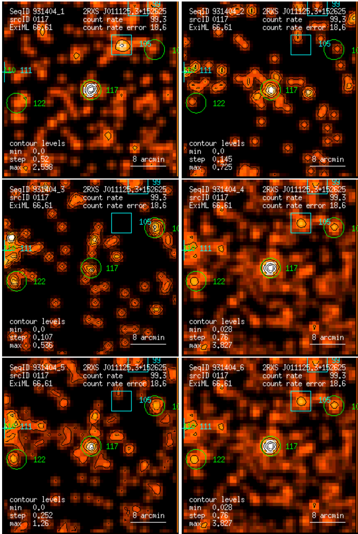
Figure 117: RASS 931404: detection 0117: band rate images, Gaussian filter: (1) PSPC channels 11 – 41, (2) 52 – 90, (3) 91 – 201, (4) 11 – 235, (5) 52 – 201, (6) 11 – 201. Broad band rates in counts/ks. Band rate contour levels in counts/ks/arcmin 2 .
